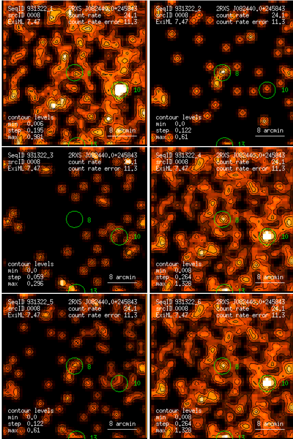
Figure 8: RASS 931322: detection 0008: band rate images, Gaussian filter: (1) PSPC channels 11 – 41, (2) 52 – 90, (3) 91 – 201, (4) 11 – 235, (5) 52 – 201, (6) 11 – 201. Broad band rates in counts/ks. Band rate contour levels in counts/ks/arcmin 2 .
