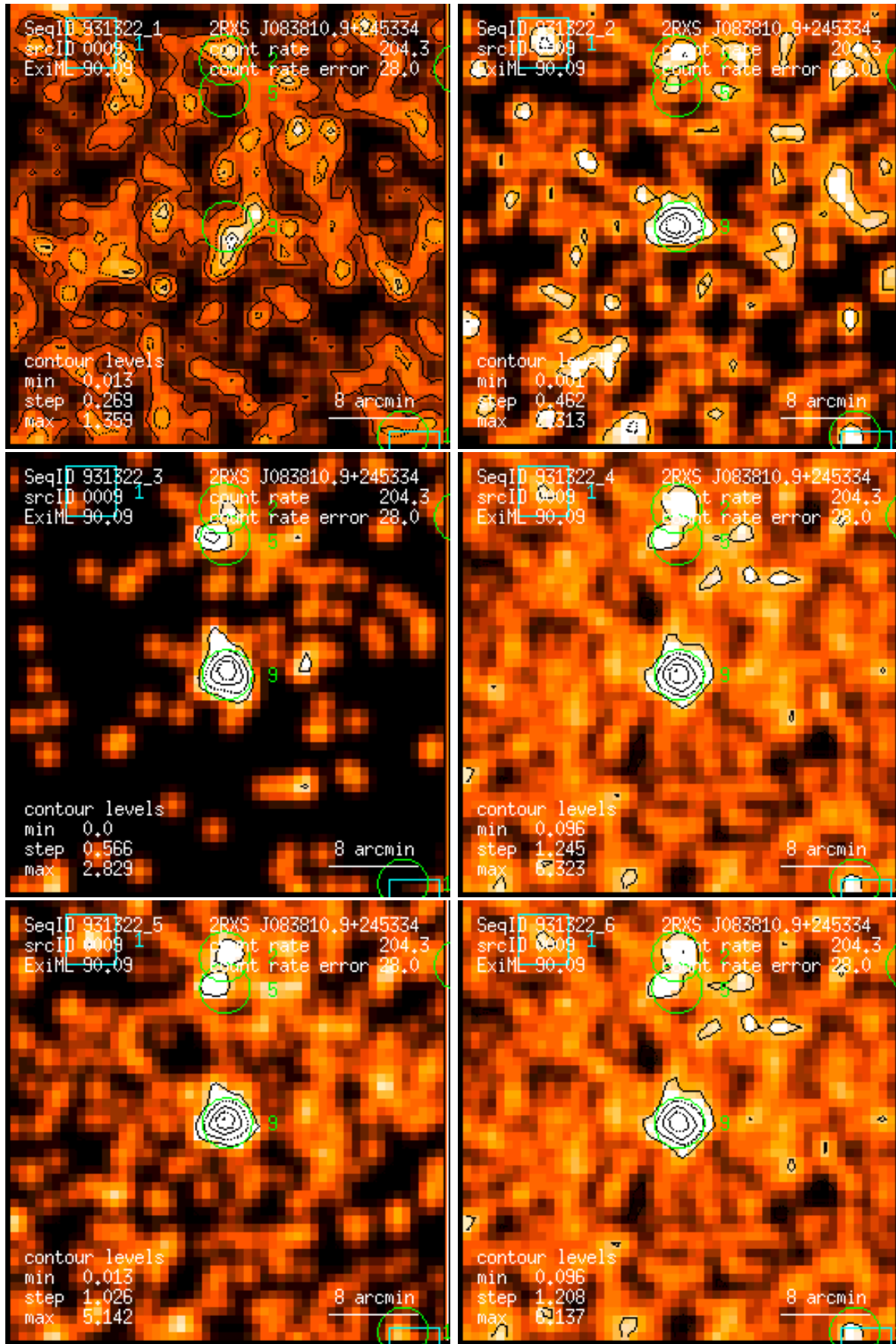
Figure 9: RASS 931322: detection 0009: band rate images, Gaussian filter: (1) PSPC channels 11 – 41, (2) 52 – 90, (3) 91 – 201, (4) 11 – 235, (5) 52 – 201, (6) 11 – 201. Broad band rates in counts/ks. Band rate contour levels in counts/ks/arcmin 2 .
