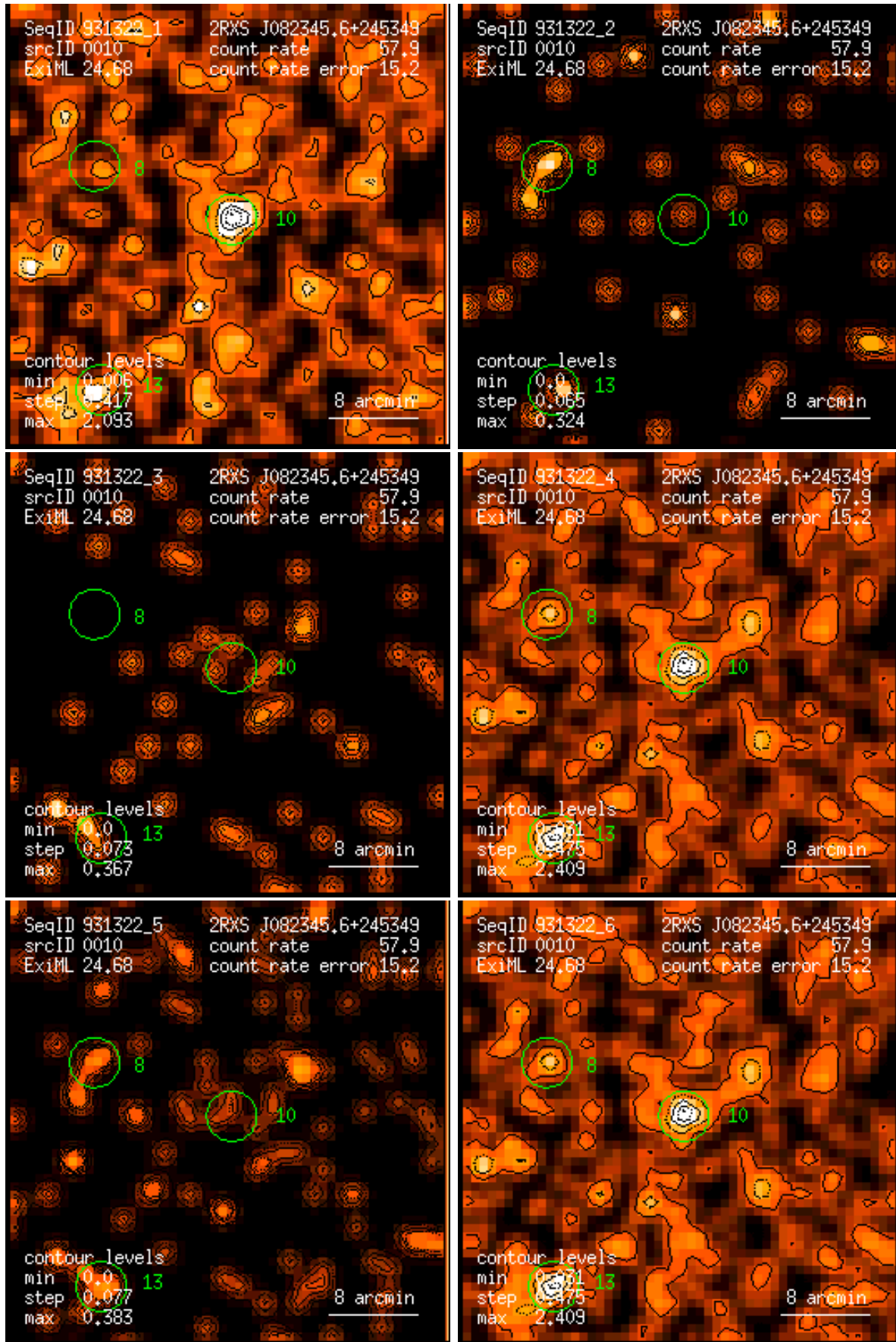
Figure 10: RASS 931322: detection 0010: band rate images, Gaussian filter: (1) PSPC channels 11 – 41, (2) 52 – 90, (3) 91 – 201, (4) 11 – 235, (5) 52 – 201, (6) 11 – 201. Broad band rates in counts/ks. Band rate contour levels in counts/ks/arcmin 2 .
