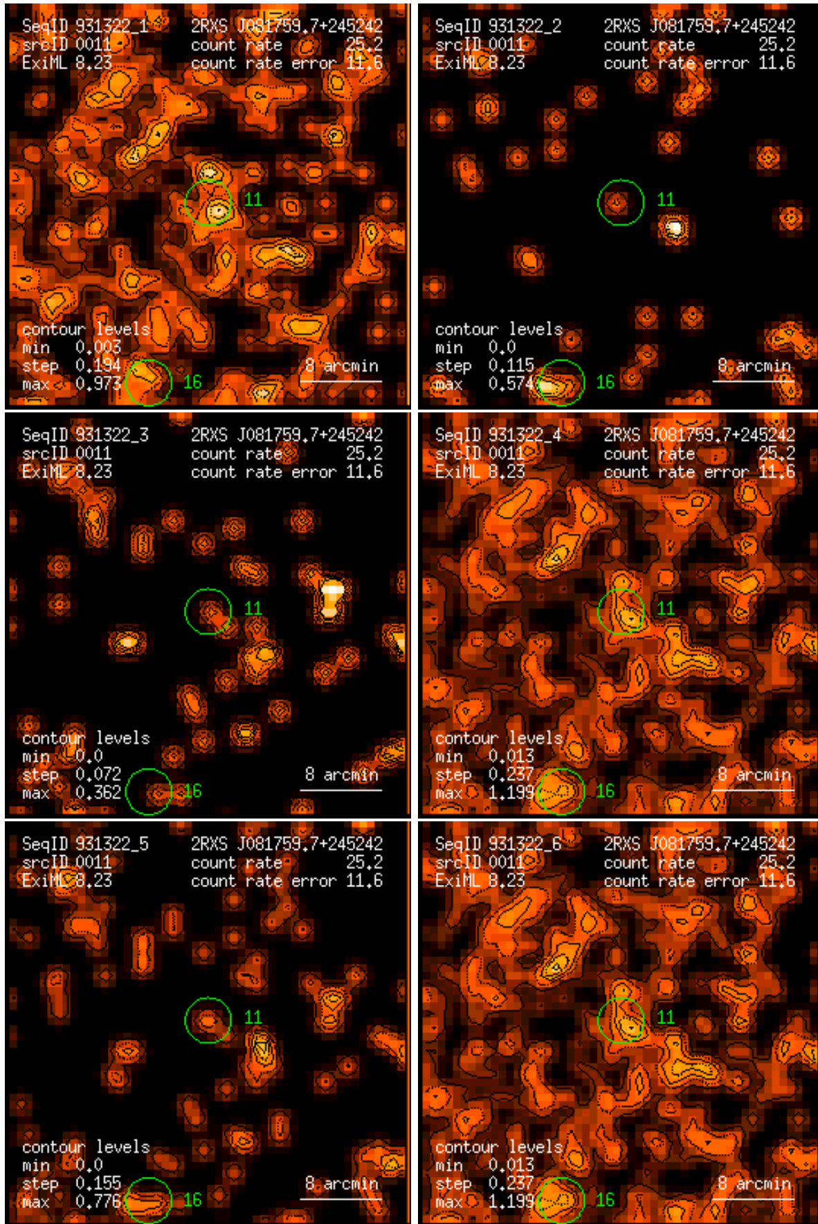
Figure 11: RASS 931322: detection 0011: band rate images, Gaussian filter: (1) PSPC channels 11 – 41, (2) 52 – 90, (3) 91 – 201, (4) 11 – 235, (5) 52 – 201, (6) 11 – 201. Broad band rates in counts/ks. Band rate contour levels in counts/ks/arcmin 2 .
