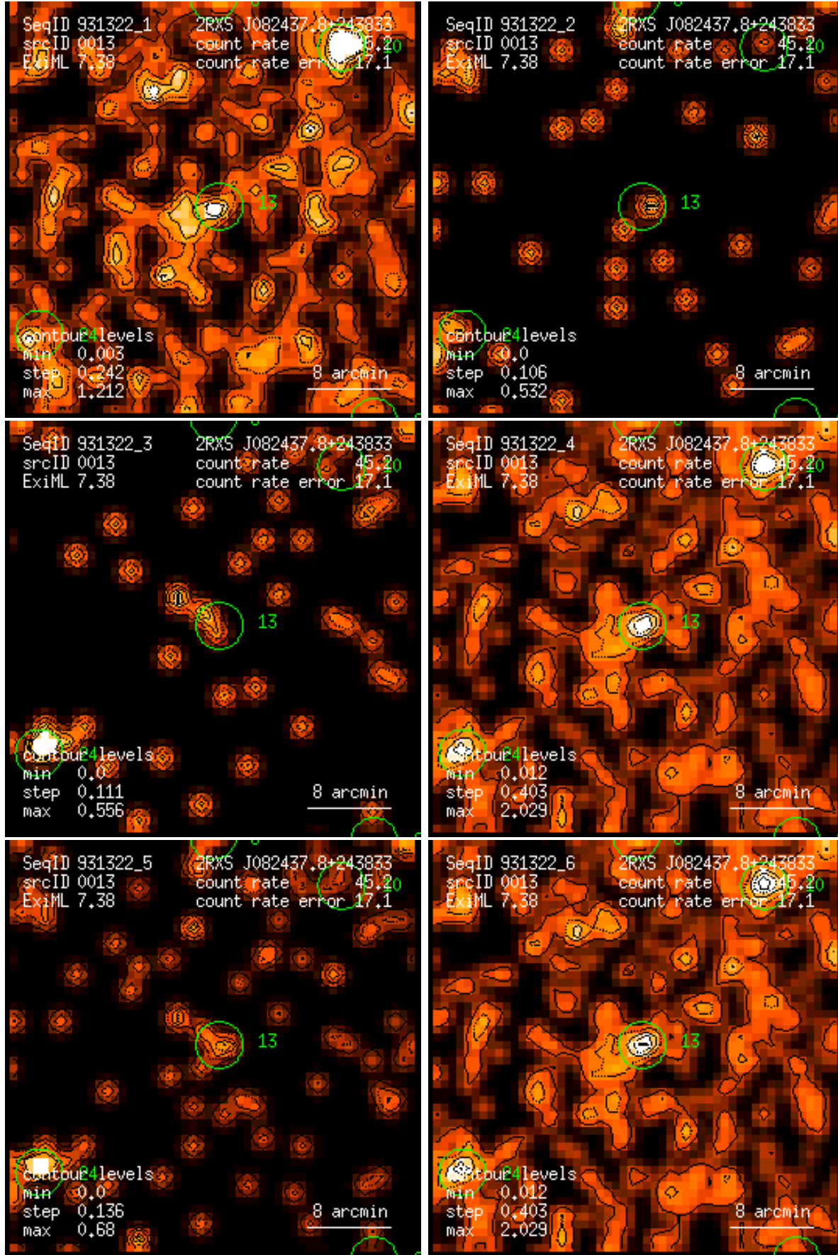
Figure 13: RASS 931322: detection 0013: band rate images, Gaussian filter: (1) PSPC channels 11 – 41, (2) 52 – 90, (3) 91 – 201, (4) 11 – 235, (5) 52 – 201, (6) 11 – 201. Broad band rates in counts/ks. Band rate contour levels in counts/ks/arcmin 2 .
