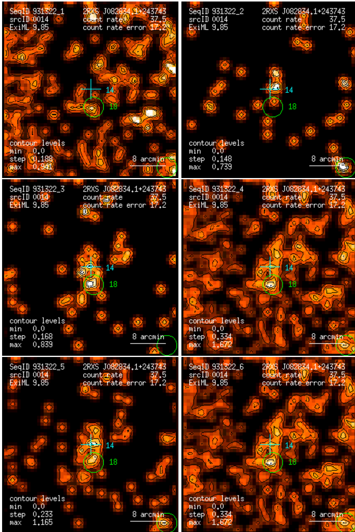
Figure 14: RASS 931322: detection 0014: band rate images, Gaussian filter: (1) PSPC channels 11 – 41, (2) 52 – 90, (3) 91 – 201, (4) 11 – 235, (5) 52 – 201, (6) 11 – 201. Broad band rates in counts/ks. Band rate contour levels in counts/ks/arcmin 2 .
