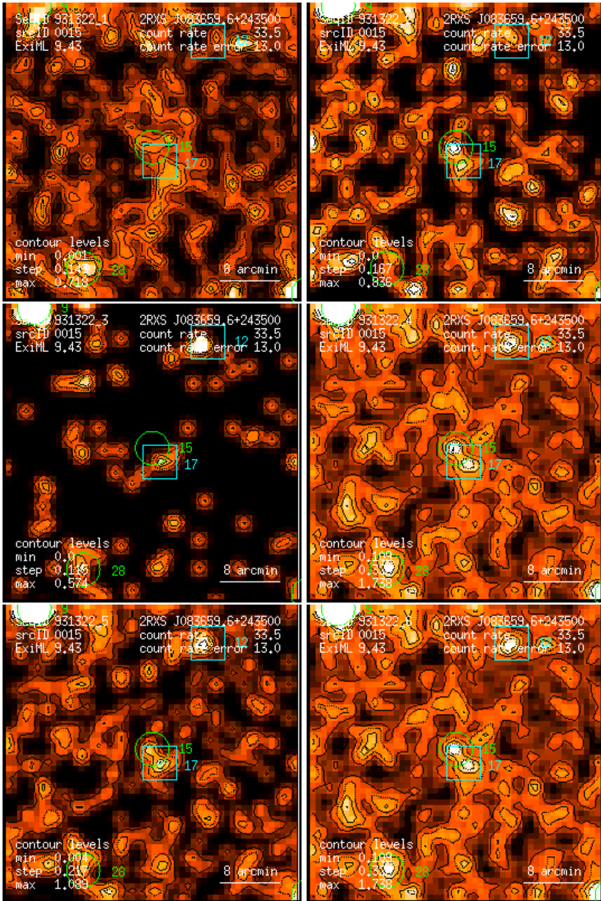
Figure 15: RASS 931322: detection 0015: band rate images, Gaussian filter: (1) PSPC channels 11 – 41, (2) 52 – 90, (3) 91 – 201, (4) 11 – 235, (5) 52 – 201, (6) 11 – 201. Broad band rates in counts/ks. Band rate contour levels in counts/ks/arcmin 2 .
