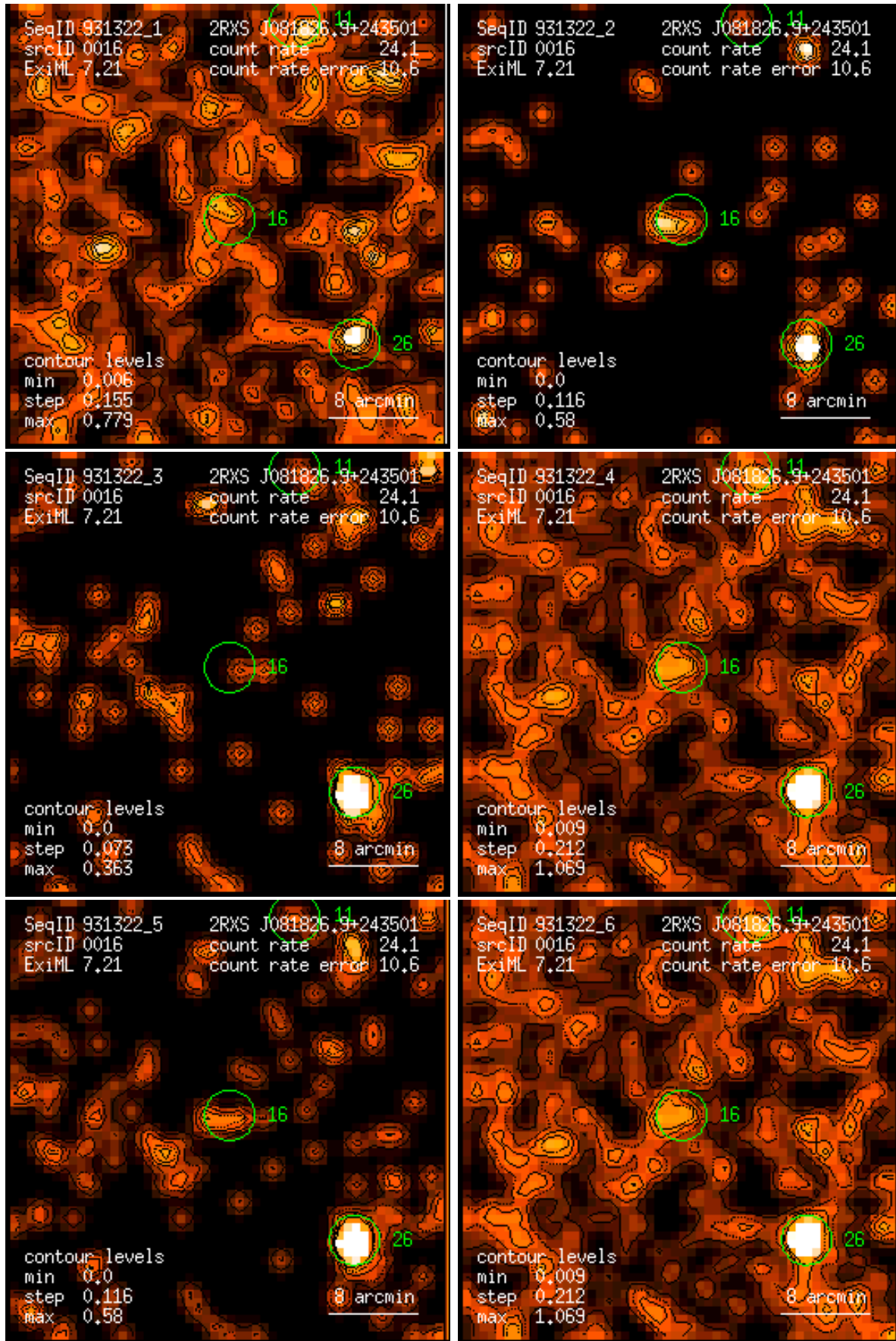
Figure 16: RASS 931322: detection 0016: band rate images, Gaussian filter: (1) PSPC channels 11 – 41, (2) 52 – 90, (3) 91 – 201, (4) 11 – 235, (5) 52 – 201, (6) 11 – 201. Broad band rates in counts/ks. Band rate contour levels in counts/ks/arcmin 2 .
