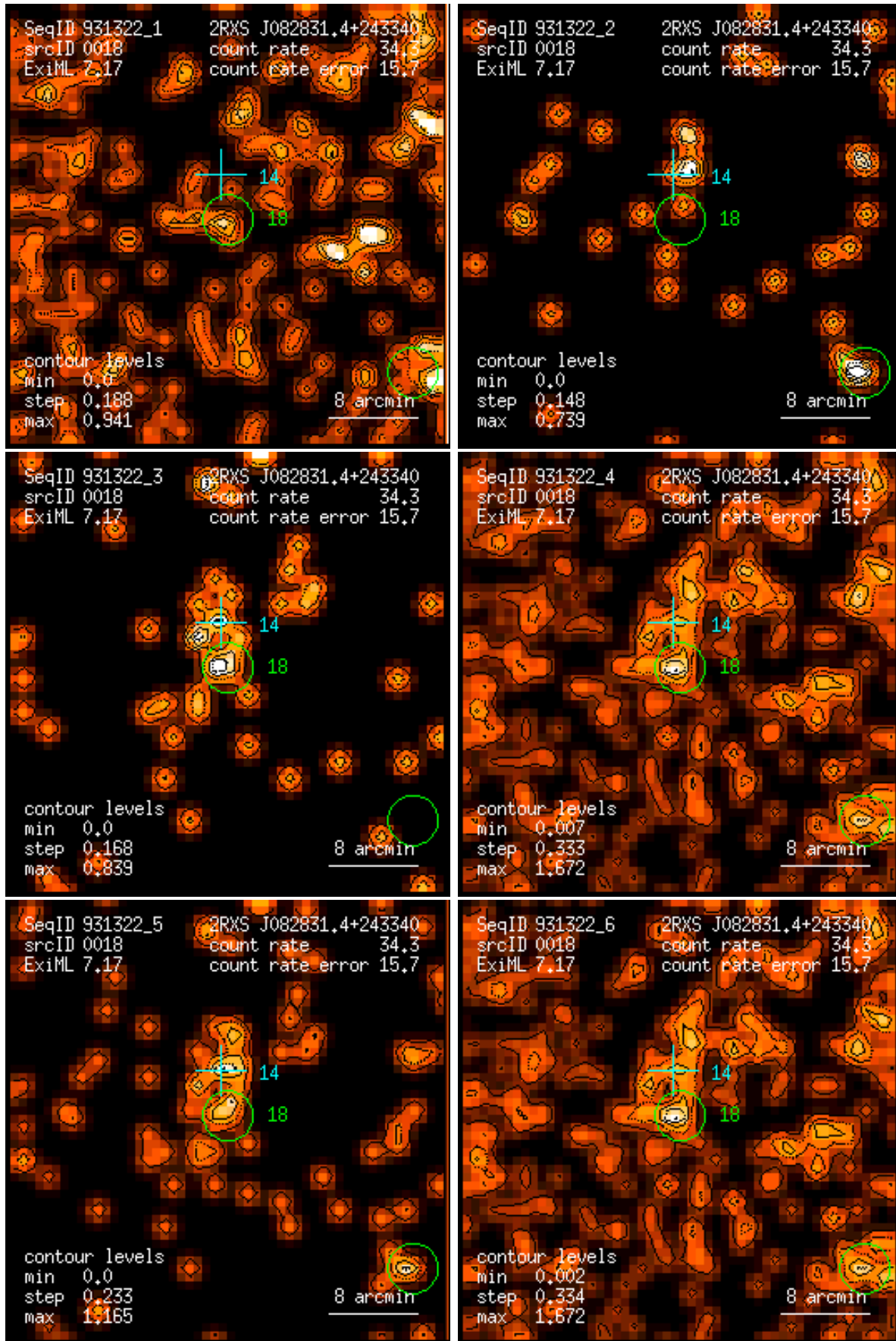
Figure 18: RASS 931322: detection 0018: band rate images, Gaussian filter: (1) PSPC channels 11 – 41, (2) 52 – 90, (3) 91 – 201, (4) 11 – 235, (5) 52 – 201, (6) 11 – 201. Broad band rates in counts/ks. Band rate contour levels in counts/ks/arcmin 2 .
