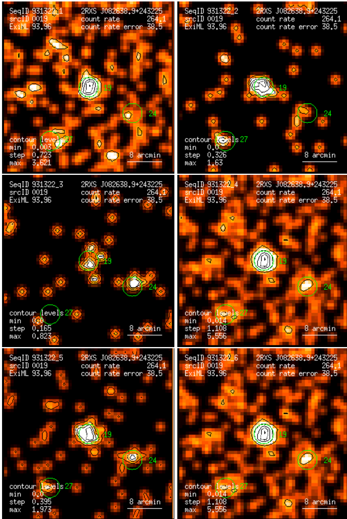
Figure 19: RASS 931322: detection 0019: band rate images, Gaussian filter: (1) PSPC channels 11 – 41, (2) 52 – 90, (3) 91 – 201, (4) 11 – 235, (5) 52 – 201, (6) 11 – 201. Broad band rates in counts/ks. Band rate contour levels in counts/ks/arcmin 2 .
