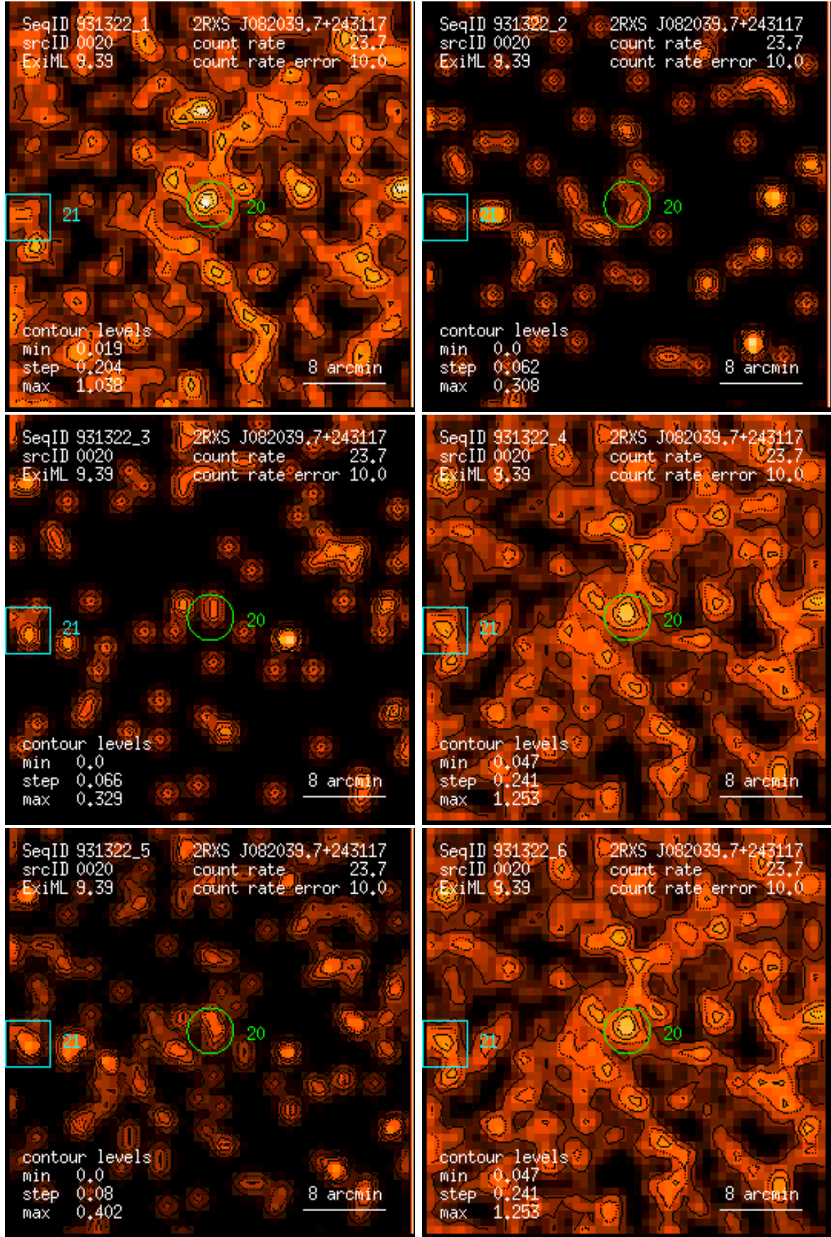
Figure 20: RASS 931322: detection 0020: band rate images, Gaussian filter: (1) PSPC channels 11 – 41, (2) 52 – 90, (3) 91 – 201, (4) 11 – 235, (5) 52 – 201, (6) 11 – 201. Broad band rates in counts/ks. Band rate contour levels in counts/ks/arcmin 2 .
