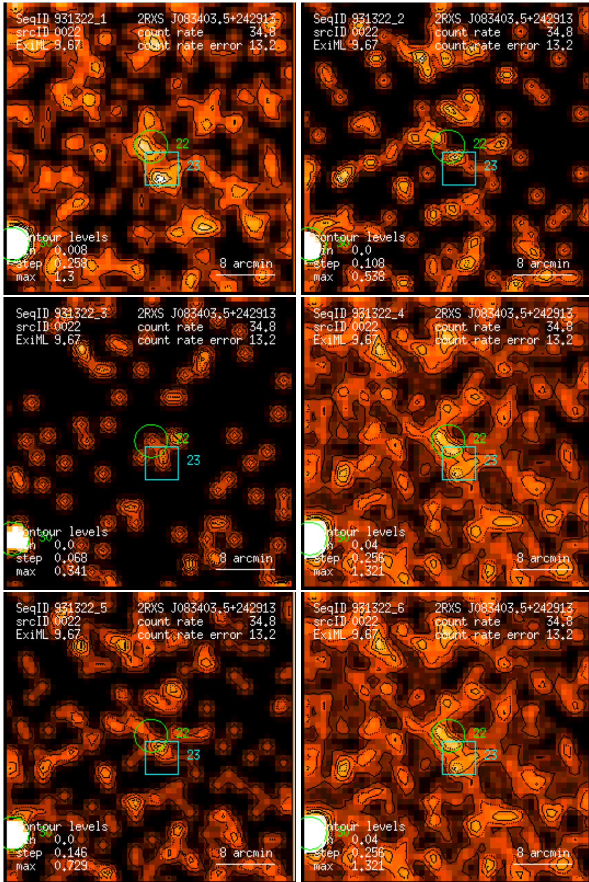
Figure 22: RASS 931322: detection 0022: band rate images, Gaussian filter: (1) PSPC channels 11 – 41, (2) 52 – 90, (3) 91 – 201, (4) 11 – 235, (5) 52 – 201, (6) 11 – 201. Broad band rates in counts/ks. Band rate contour levels in counts/ks/arcmin 2 .
