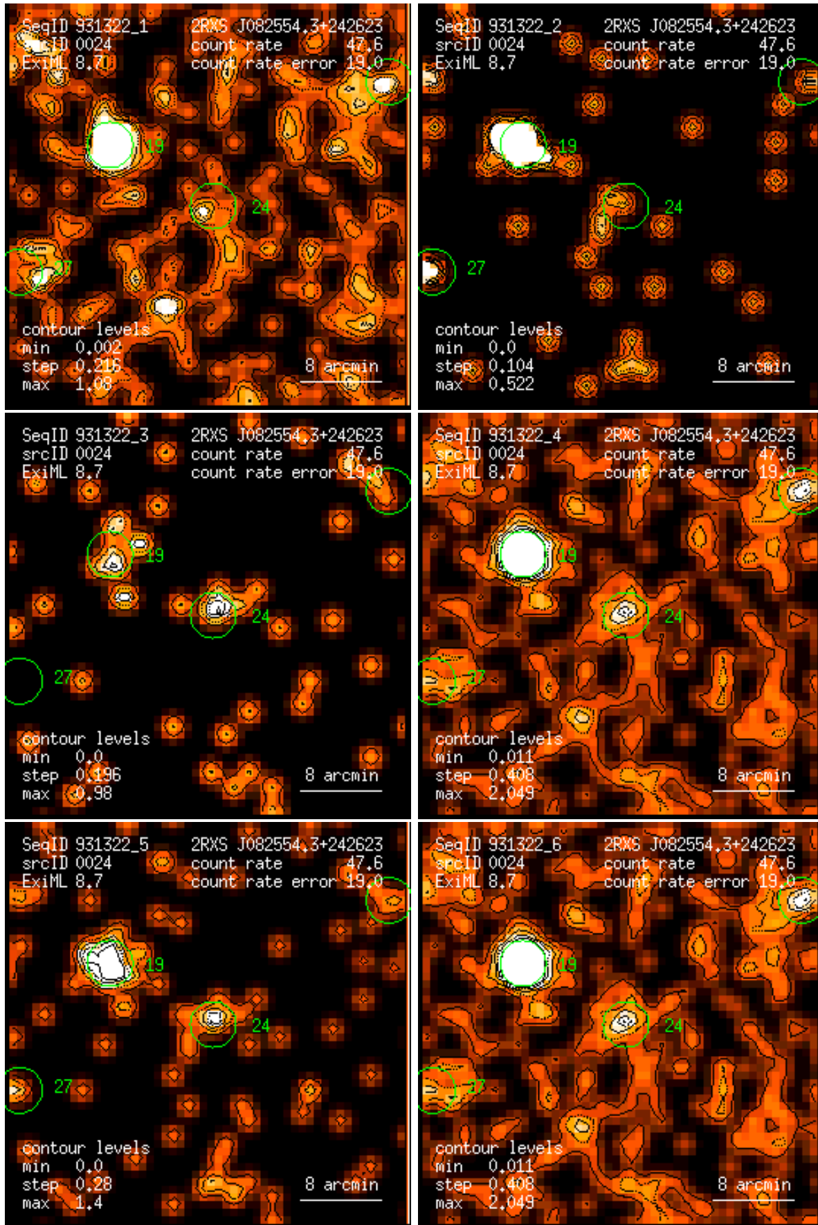
Figure 24: RASS 931322: detection 0024: band rate images, Gaussian filter: (1) PSPC channels 11 – 41, (2) 52 – 90, (3) 91 – 201, (4) 11 – 235, (5) 52 – 201, (6) 11 – 201. Broad band rates in counts/ks. Band rate contour levels in counts/ks/arcmin 2 .
