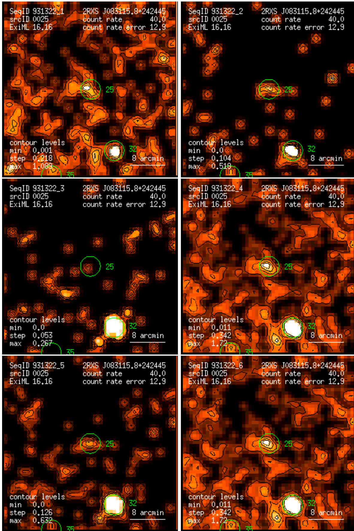
Figure 25: RASS 931322: detection 0025: band rate images, Gaussian filter: (1) PSPC channels 11 – 41, (2) 52 – 90, (3) 91 – 201, (4) 11 – 235, (5) 52 – 201, (6) 11 – 201. Broad band rates in counts/ks. Band rate contour levels in counts/ks/arcmin 2 .
