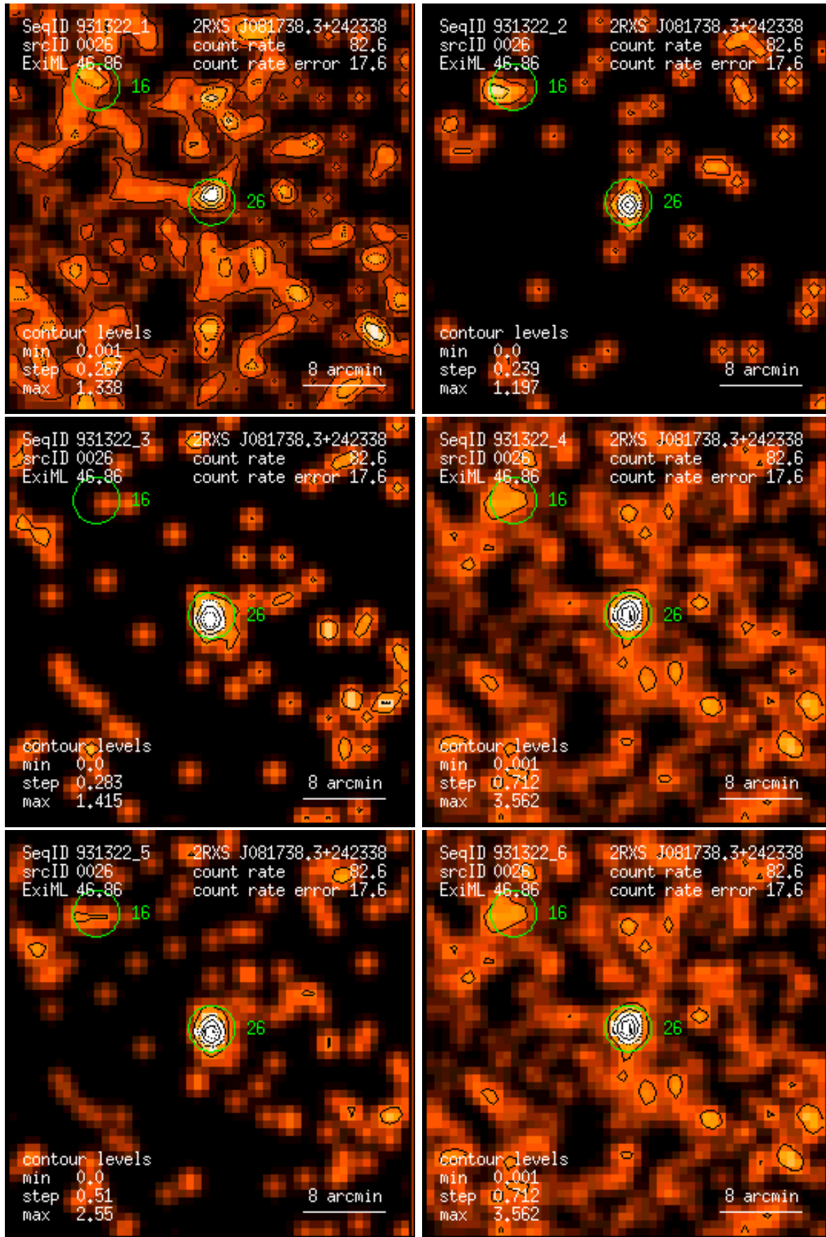
Figure 26: RASS 931322: detection 0026: band rate images, Gaussian filter: (1) PSPC channels 11 – 41, (2) 52 – 90, (3) 91 – 201, (4) 11 – 235, (5) 52 – 201, (6) 11 – 201. Broad band rates in counts/ks. Band rate contour levels in counts/ks/arcmin 2 .
