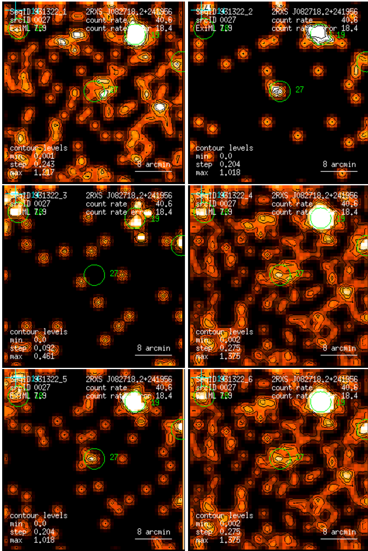
Figure 27: RASS 931322: detection 0027: band rate images, Gaussian filter: (1) PSPC channels 11 – 41, (2) 52 – 90, (3) 91 – 201, (4) 11 – 235, (5) 52 – 201, (6) 11 – 201. Broad band rates in counts/ks. Band rate contour levels in counts/ks/arcmin 2 .
