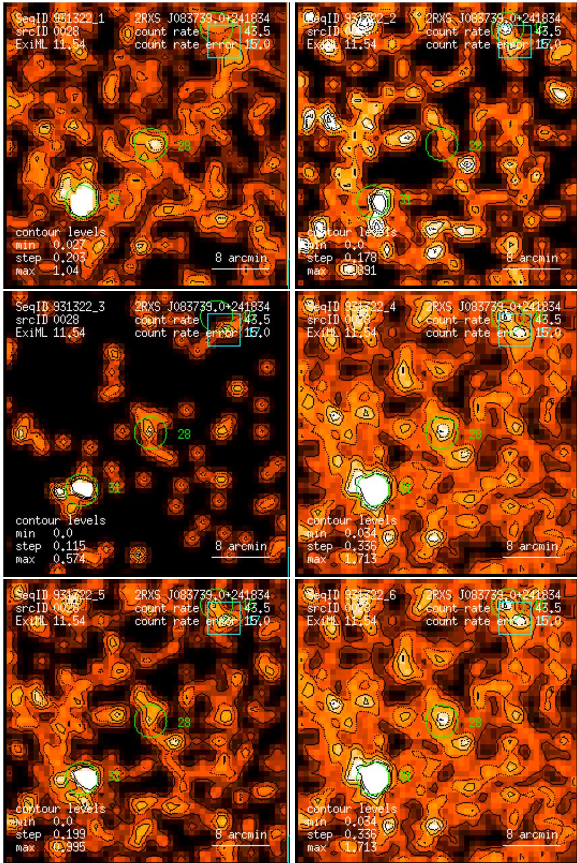
Figure 28: RASS 931322: detection 0028: band rate images, Gaussian filter: (1) PSPC channels 11 – 41, (2) 52 – 90, (3) 91 – 201, (4) 11 – 235, (5) 52 – 201, (6) 11 – 201. Broad band rates in counts/ks. Band rate contour levels in counts/ks/arcmin 2 .
