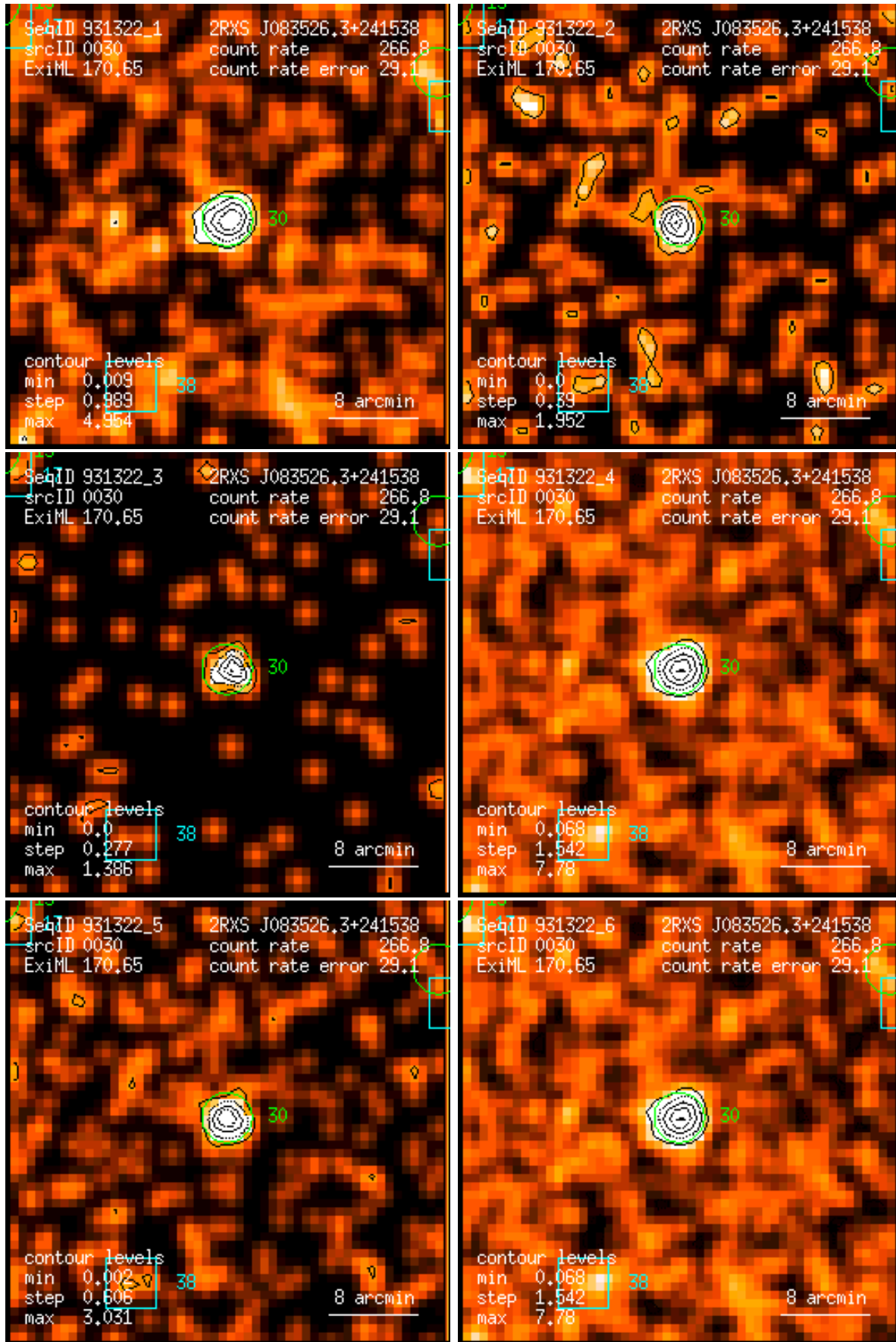
Figure 30: RASS 931322: detection 0030: band rate images, Gaussian filter: (1) PSPC channels 11 – 41, (2) 52 – 90, (3) 91 – 201, (4) 11 – 235, (5) 52 – 201, (6) 11 – 201. Broad band rates in counts/ks. Band rate contour levels in counts/ks/arcmin 2 .
