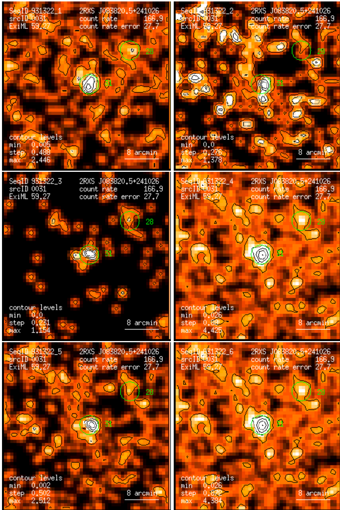
Figure 31: RASS 931322: detection 0031: band rate images, Gaussian filter: (1) PSPC channels 11 – 41, (2) 52 – 90, (3) 91 – 201, (4) 11 – 235, (5) 52 – 201, (6) 11 – 201. Broad band rates in counts/ks. Band rate contour levels in counts/ks/arcmin 2 .
