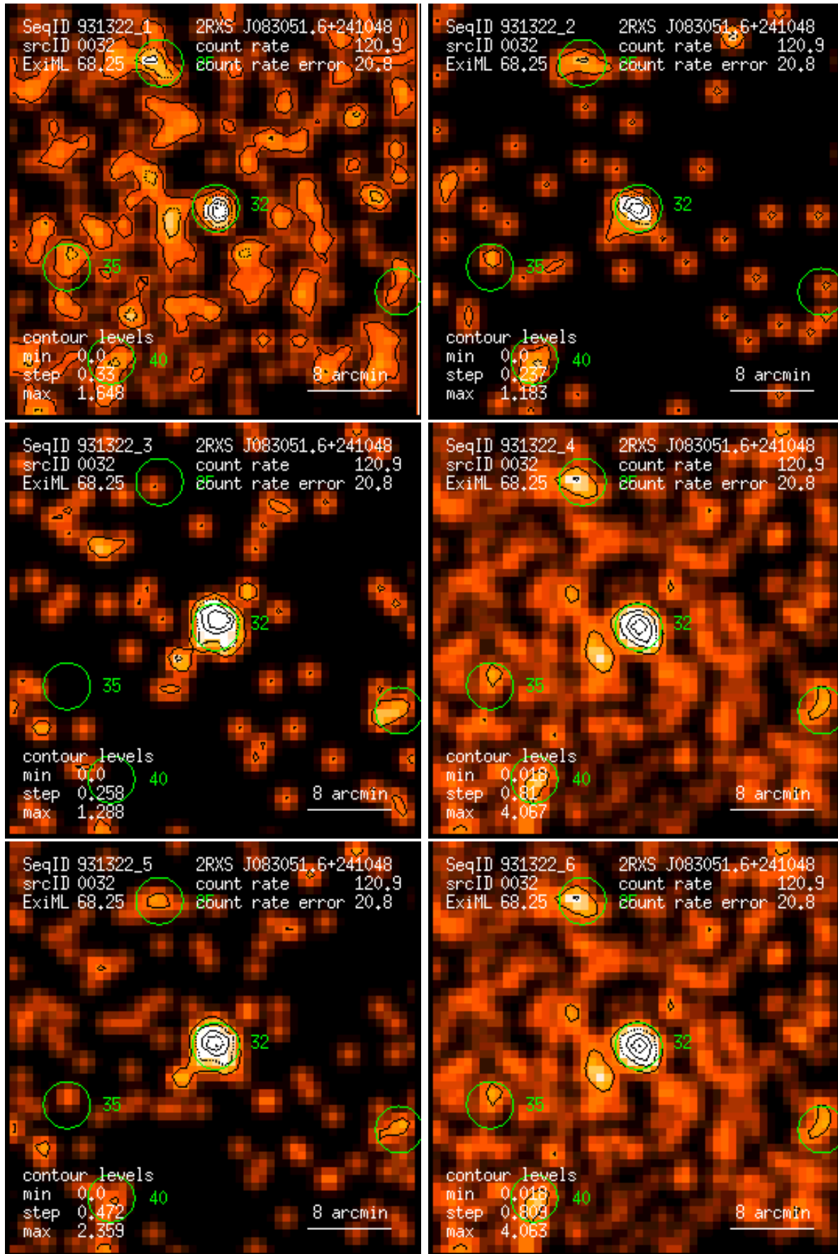
Figure 32: RASS 931322: detection 0032: band rate images, Gaussian filter: (1) PSPC channels 11 – 41, (2) 52 – 90, (3) 91 – 201, (4) 11 – 235, (5) 52 – 201, (6) 11 – 201. Broad band rates in counts/ks. Band rate contour levels in counts/ks/arcmin 2 .
