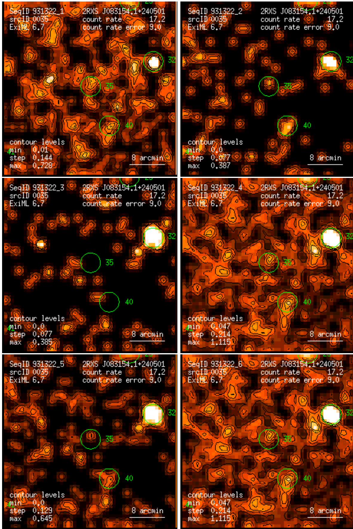
Figure 35: RASS 931322: detection 0035: band rate images, Gaussian filter: (1) PSPC channels 11 – 41, (2) 52 – 90, (3) 91 – 201, (4) 11 – 235, (5) 52 – 201, (6) 11 – 201. Broad band rates in counts/ks. Band rate contour levels in counts/ks/arcmin 2 .
