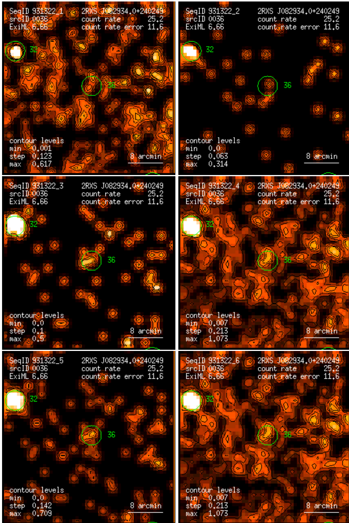
Figure 36: RASS 931322: detection 0036: band rate images, Gaussian filter: (1) PSPC channels 11 – 41, (2) 52 – 90, (3) 91 – 201, (4) 11 – 235, (5) 52 – 201, (6) 11 – 201. Broad band rates in counts/ks. Band rate contour levels in counts/ks/arcmin 2 .
