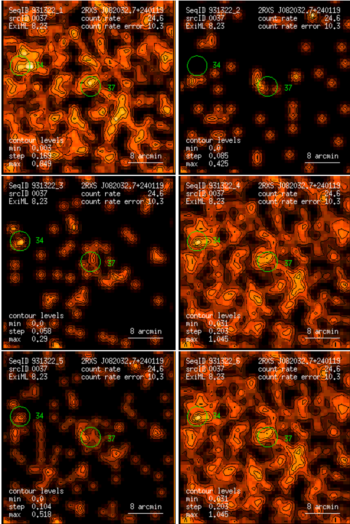
Figure 37: RASS 931322: detection 0037: band rate images, Gaussian filter: (1) PSPC channels 11 – 41, (2) 52 – 90, (3) 91 – 201, (4) 11 – 235, (5) 52 – 201, (6) 11 – 201. Broad band rates in counts/ks. Band rate contour levels in counts/ks/arcmin 2 .
