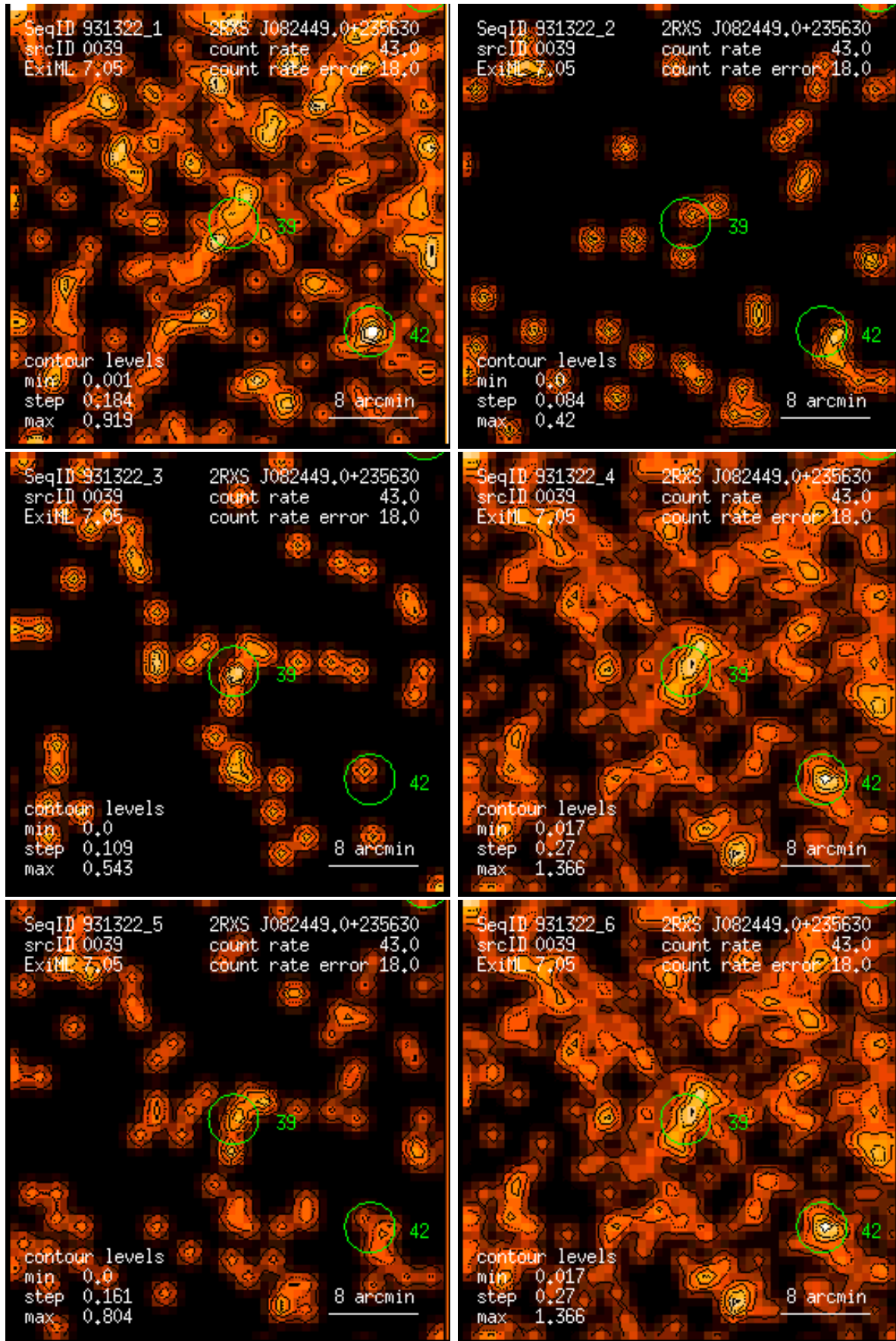
Figure 39: RASS 931322: detection 0039: band rate images, Gaussian filter: (1) PSPC channels 11 – 41, (2) 52 – 90, (3) 91 – 201, (4) 11 – 235, (5) 52 – 201, (6) 11 – 201. Broad band rates in counts/ks. Band rate contour levels in counts/ks/arcmin 2 .
