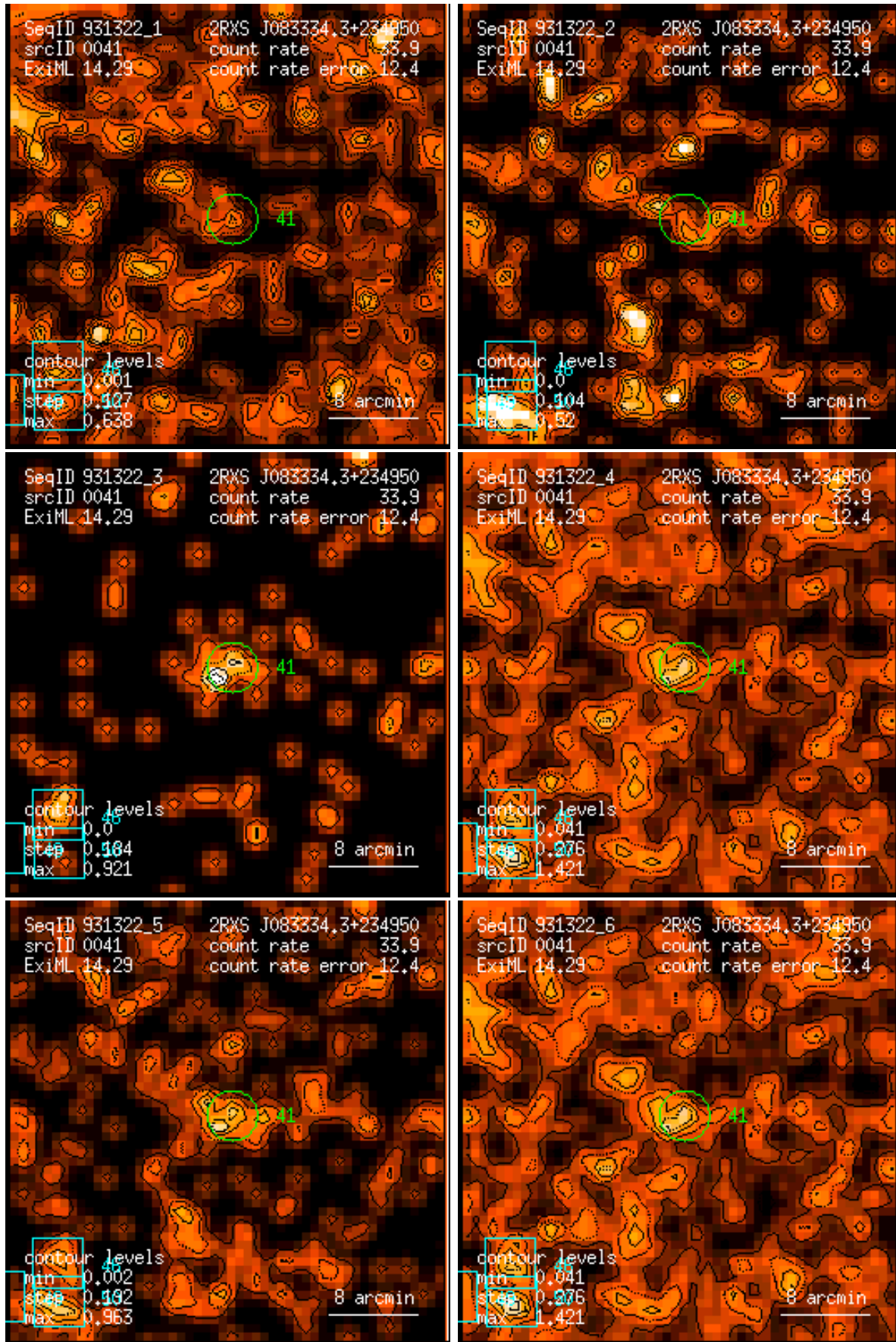
Figure 41: RASS 931322: detection 0041: band rate images, Gaussian filter: (1) PSPC channels 11 – 41, (2) 52 – 90, (3) 91 – 201, (4) 11 – 235, (5) 52 – 201, (6) 11 – 201. Broad band rates in counts/ks. Band rate contour levels in counts/ks/arcmin 2 .
