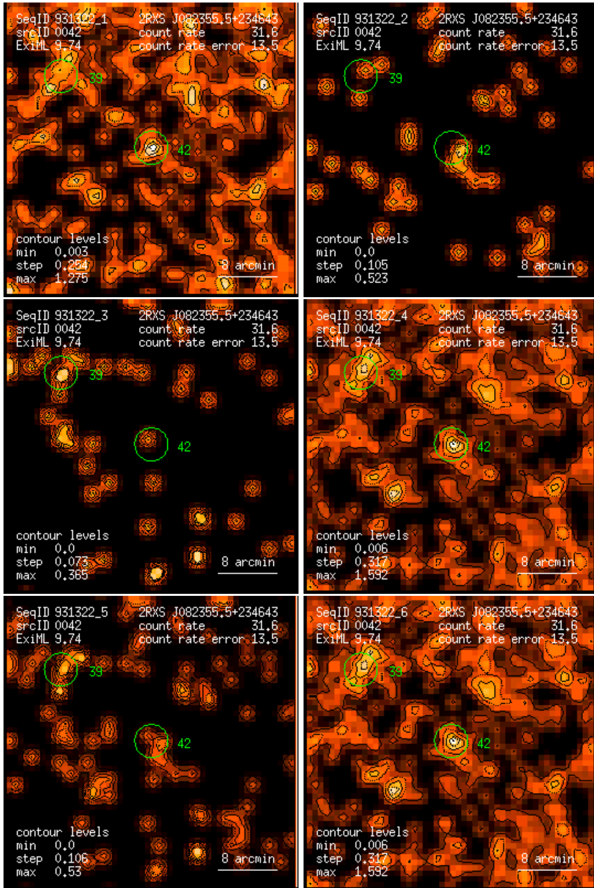
Figure 42: RASS 931322: detection 0042: band rate images, Gaussian filter: (1) PSPC channels 11 – 41, (2) 52 – 90, (3) 91 – 201, (4) 11 – 235, (5) 52 – 201, (6) 11 – 201. Broad band rates in counts/ks. Band rate contour levels in counts/ks/arcmin 2 .
