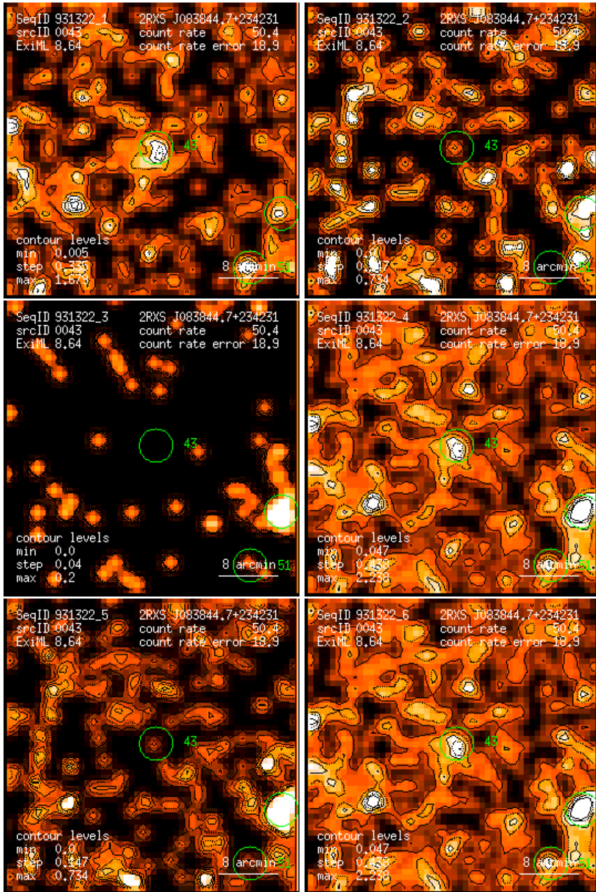
Figure 43: RASS 931322: detection 0043: band rate images, Gaussian filter: (1) PSPC channels 11 – 41, (2) 52 – 90, (3) 91 – 201, (4) 11 – 235, (5) 52 – 201, (6) 11 – 201. Broad band rates in counts/ks. Band rate contour levels in counts/ks/arcmin 2 .
