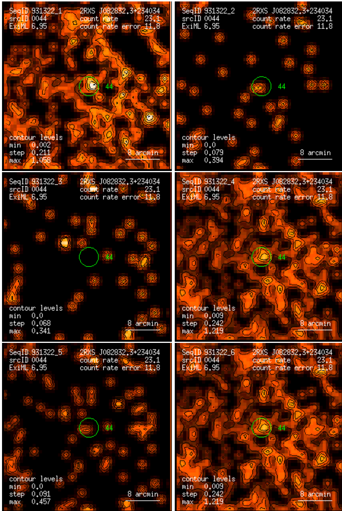
Figure 44: RASS 931322: detection 0044: band rate images, Gaussian filter: (1) PSPC channels 11 – 41, (2) 52 – 90, (3) 91 – 201, (4) 11 – 235, (5) 52 – 201, (6) 11 – 201. Broad band rates in counts/ks. Band rate contour levels in counts/ks/arcmin 2 .
