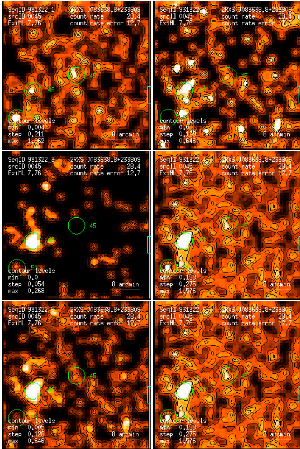
Figure 45: RASS 931322: detection 0045: band rate images, Gaussian filter: (1) PSPC channels 11 – 41, (2) 52 – 90, (3) 91 – 201, (4) 11 – 235, (5) 52 – 201, (6) 11 – 201. Broad band rates in counts/ks. Band rate contour levels in counts/ks/arcmin 2 .
