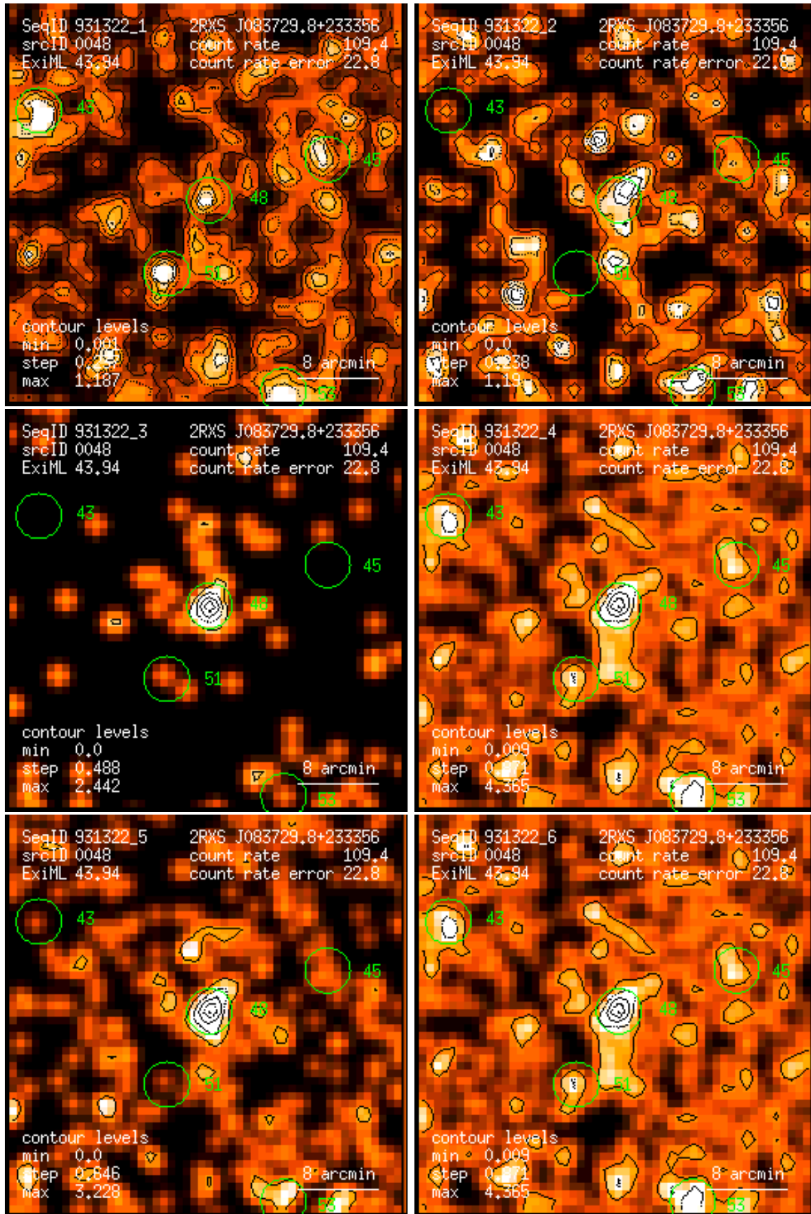
Figure 48: RASS 931322: detection 0048: band rate images, Gaussian filter: (1) PSPC channels 11 – 41, (2) 52 – 90, (3) 91 – 201, (4) 11 – 235, (5) 52 – 201, (6) 11 – 201. Broad band rates in counts/ks. Band rate contour levels in counts/ks/arcmin 2 .
