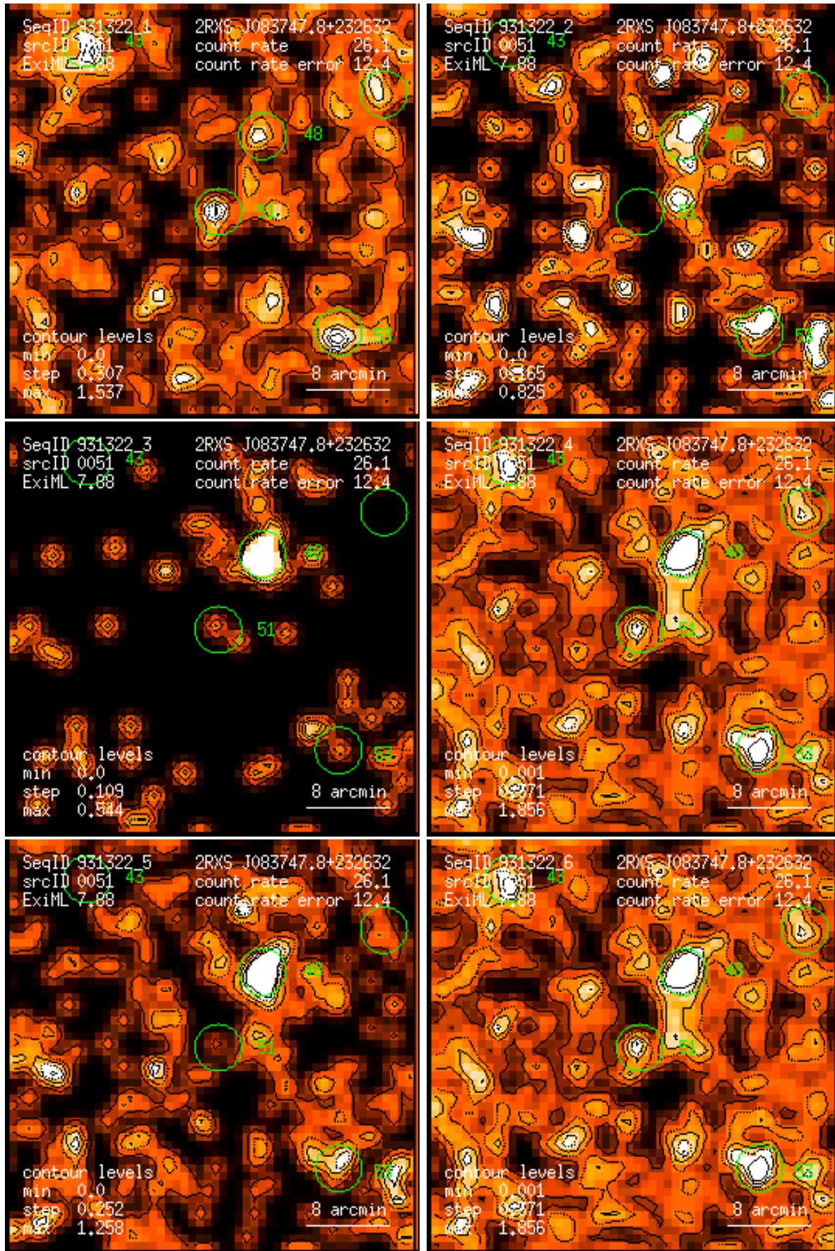
Figure 51: RASS 931322: detection 0051: band rate images, Gaussian filter: (1) PSPC channels 11 – 41, (2) 52 – 90, (3) 91 – 201, (4) 11 – 235, (5) 52 – 201, (6) 11 – 201. Broad band rates in counts/ks. Band rate contour levels in counts/ks/arcmin 2 .
