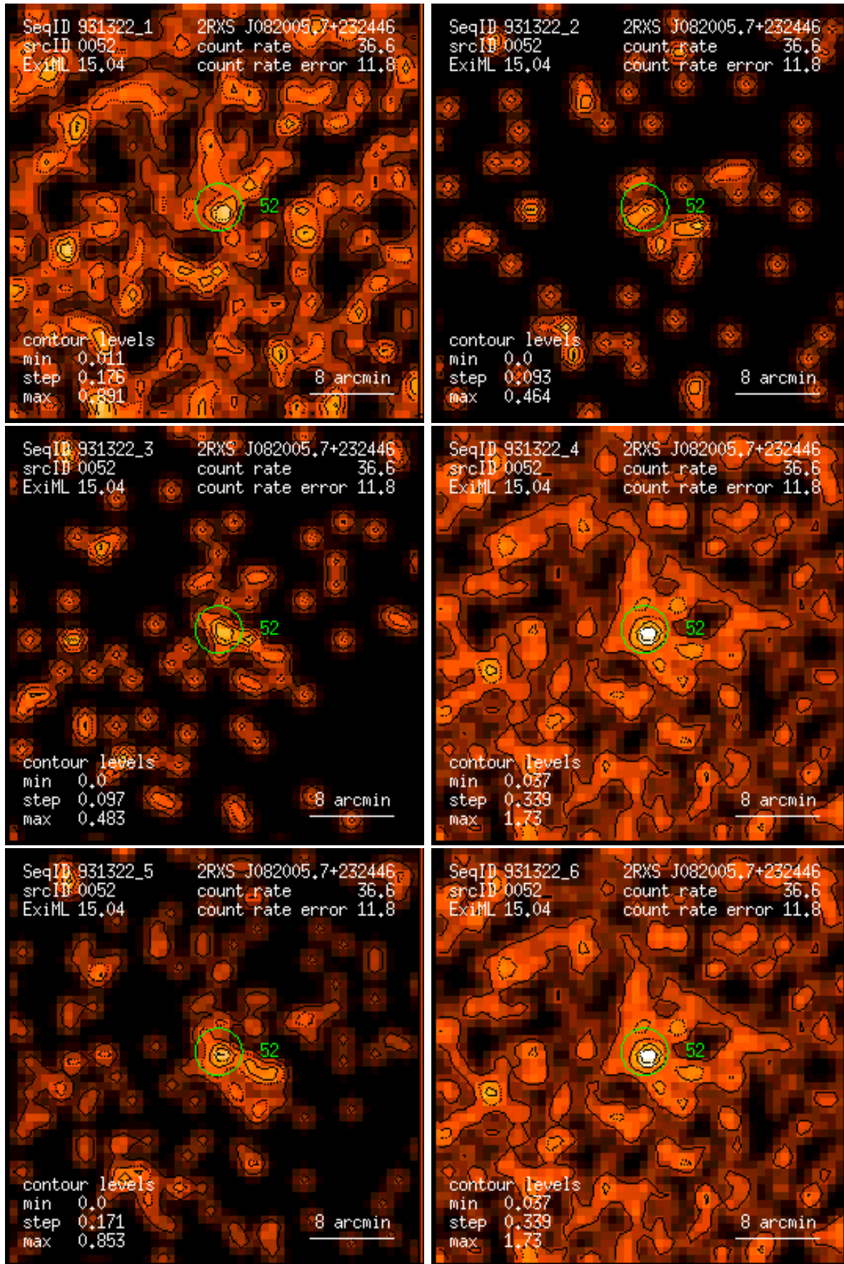
Figure 52: RASS 931322: detection 0052: band rate images, Gaussian filter: (1) PSPC channels 11 – 41, (2) 52 – 90, (3) 91 – 201, (4) 11 – 235, (5) 52 – 201, (6) 11 – 201. Broad band rates in counts/ks. Band rate contour levels in counts/ks/arcmin 2 .
