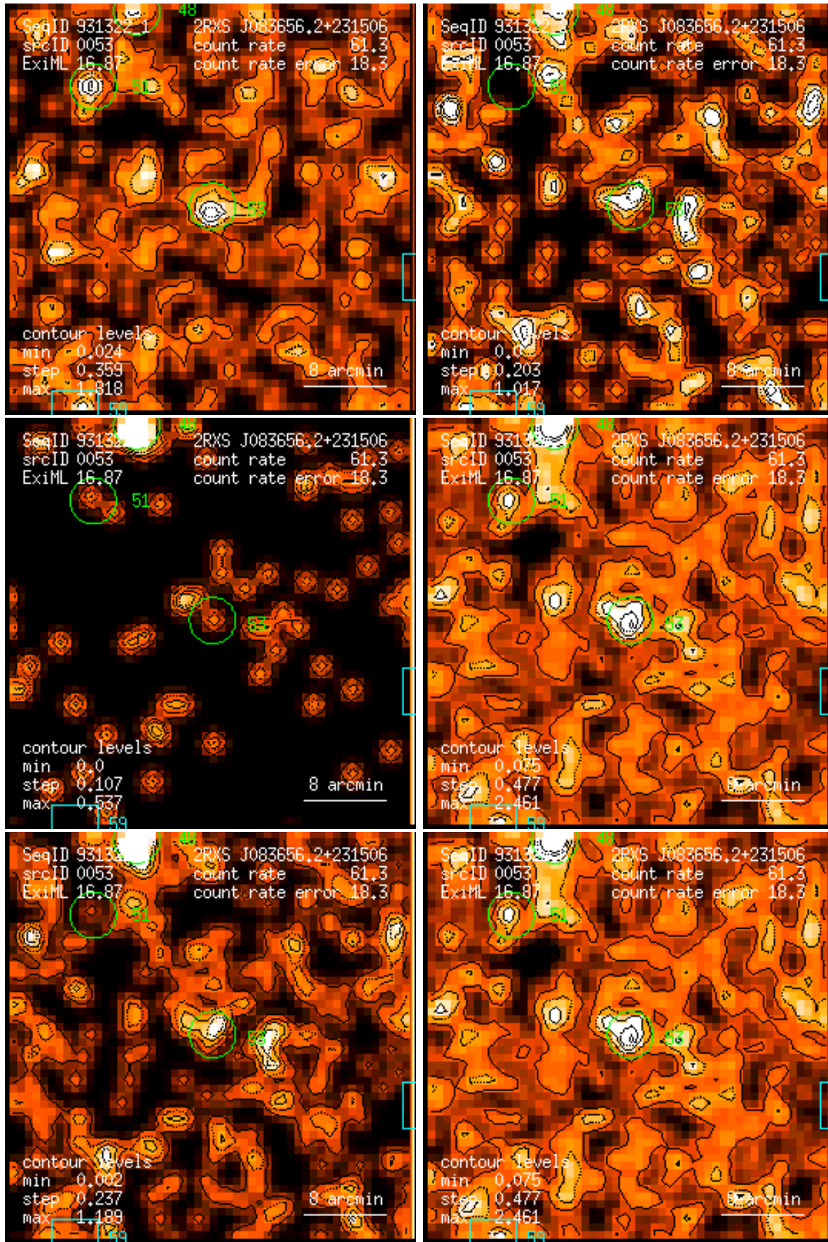
Figure 53: RASS 931322: detection 0053: band rate images, Gaussian filter: (1) PSPC channels 11 – 41, (2) 52 – 90, (3) 91 – 201, (4) 11 – 235, (5) 52 – 201, (6) 11 – 201. Broad band rates in counts/ks. Band rate contour levels in counts/ks/arcmin 2 .
