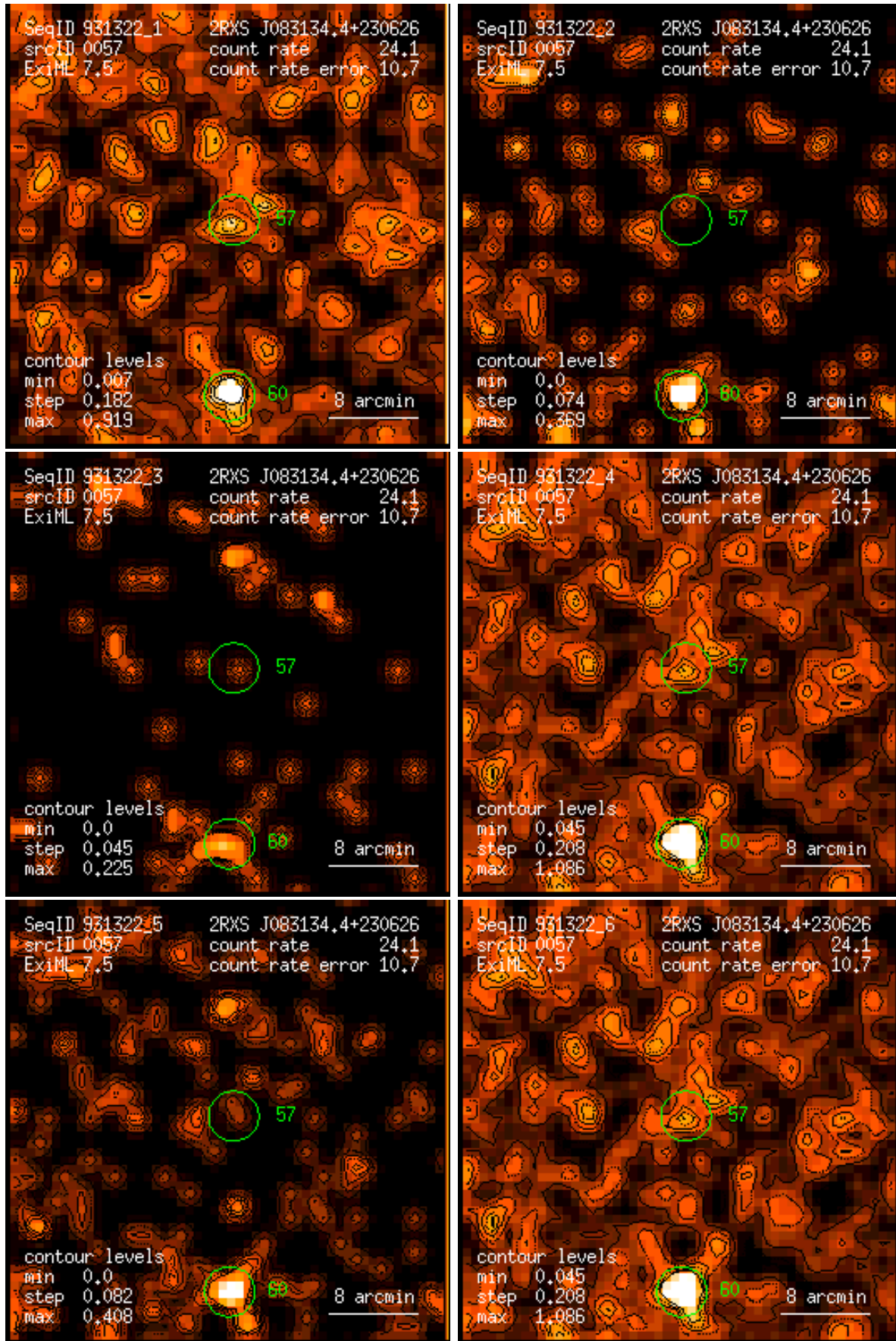
Figure 57: RASS 931322: detection 0057: band rate images, Gaussian filter: (1) PSPC channels 11 – 41, (2) 52 – 90, (3) 91 – 201, (4) 11 – 235, (5) 52 – 201, (6) 11 – 201. Broad band rates in counts/ks. Band rate contour levels in counts/ks/arcmin 2 .
