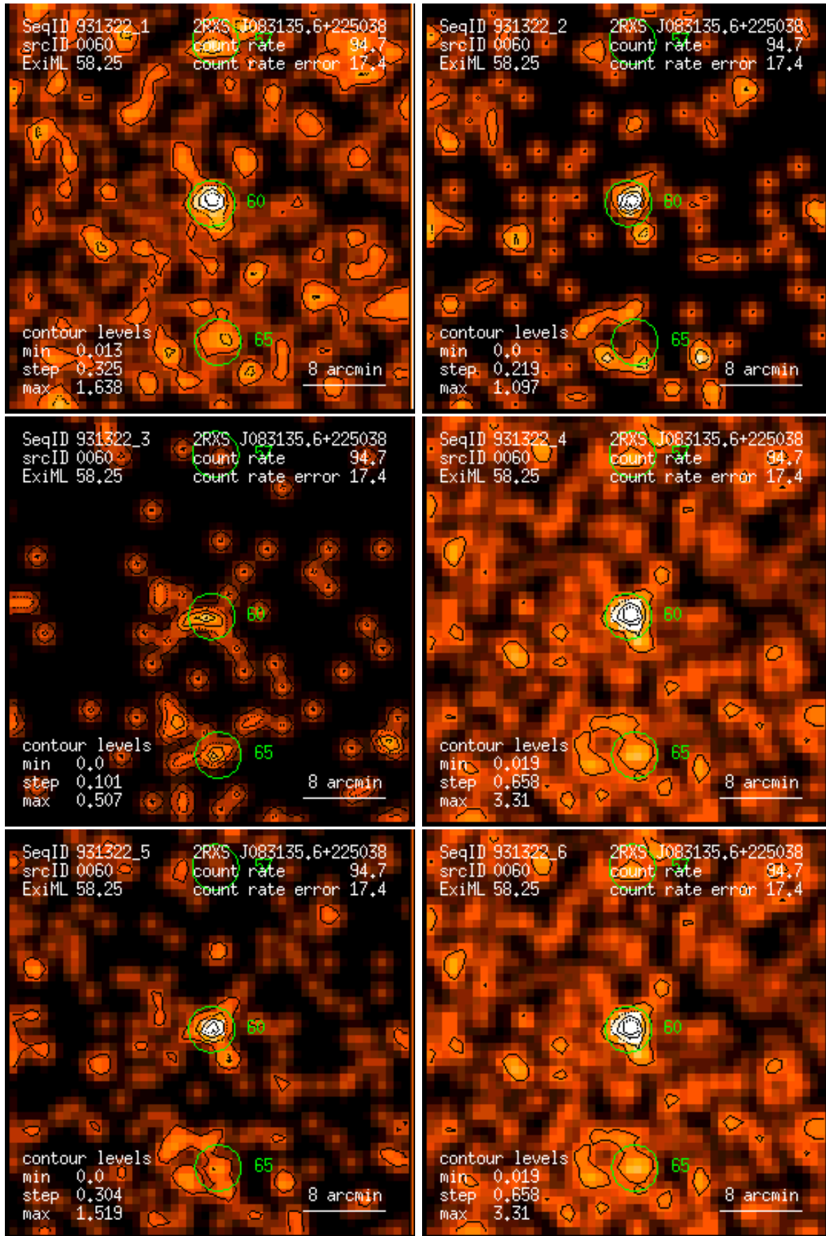
Figure 60: RASS 931322: detection 0060: band rate images, Gaussian filter: (1) PSPC channels 11 – 41, (2) 52 – 90, (3) 91 – 201, (4) 11 – 235, (5) 52 – 201, (6) 11 – 201. Broad band rates in counts/ks. Band rate contour levels in counts/ks/arcmin 2 .
