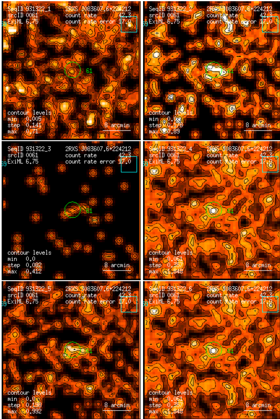
Figure 61: RASS 931322: detection 0061: band rate images, Gaussian filter: (1) PSPC channels 11 – 41, (2) 52 – 90, (3) 91 – 201, (4) 11 – 235, (5) 52 – 201, (6) 11 – 201. Broad band rates in counts/ks. Band rate contour levels in counts/ks/arcmin 2 .
