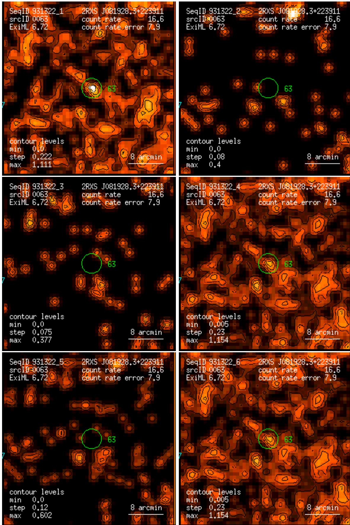
Figure 63: RASS 931322: detection 0063: band rate images, Gaussian filter: (1) PSPC channels 11 – 41, (2) 52 – 90, (3) 91 – 201, (4) 11 – 235, (5) 52 – 201, (6) 11 – 201. Broad band rates in counts/ks. Band rate contour levels in counts/ks/arcmin 2 .
