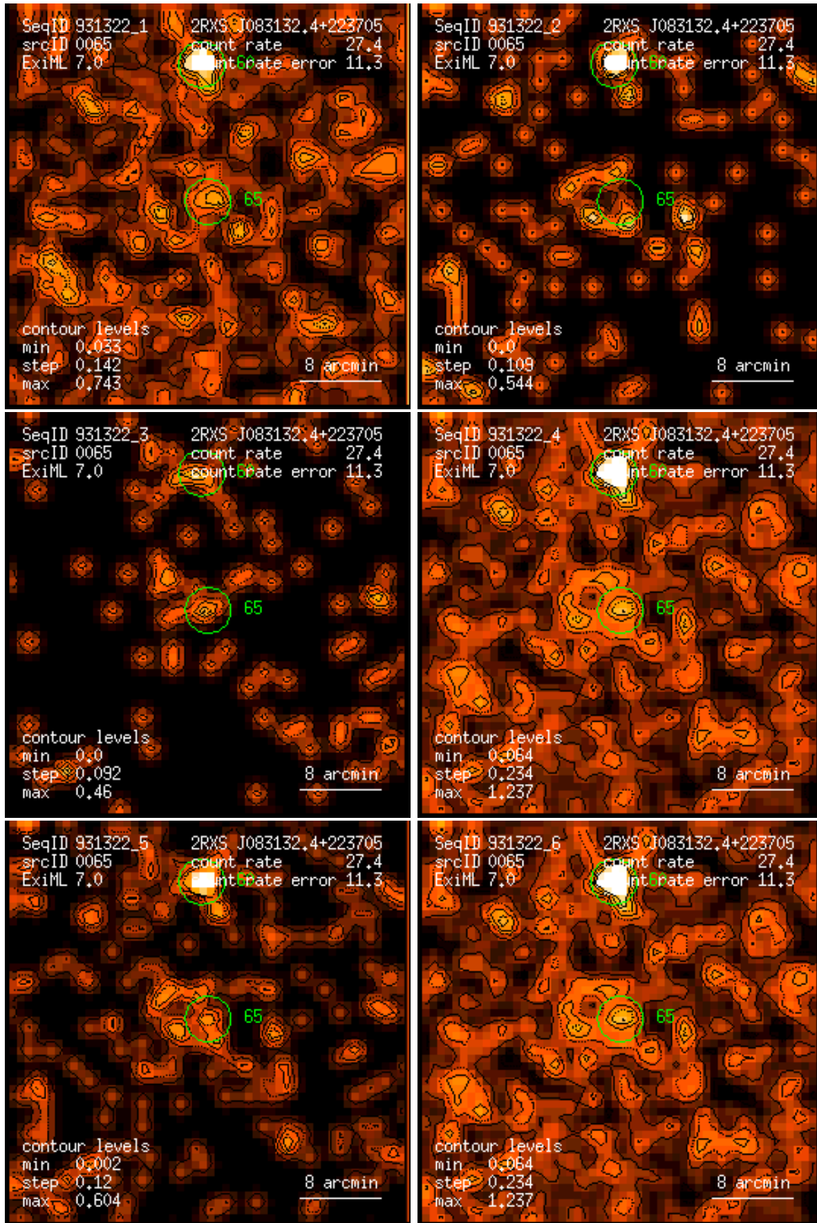
Figure 65: RASS 931322: detection 0065: band rate images, Gaussian filter: (1) PSPC channels 11 – 41, (2) 52 – 90, (3) 91 – 201, (4) 11 – 235, (5) 52 – 201, (6) 11 – 201. Broad band rates in counts/ks. Band rate contour levels in counts/ks/arcmin 2 .
