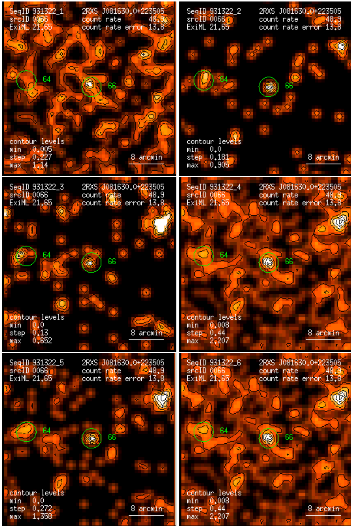
Figure 66: RASS 931322: detection 0066: band rate images, Gaussian filter: (1) PSPC channels 11 – 41, (2) 52 – 90, (3) 91 – 201, (4) 11 – 235, (5) 52 – 201, (6) 11 – 201. Broad band rates in counts/ks. Band rate contour levels in counts/ks/arcmin 2 .
