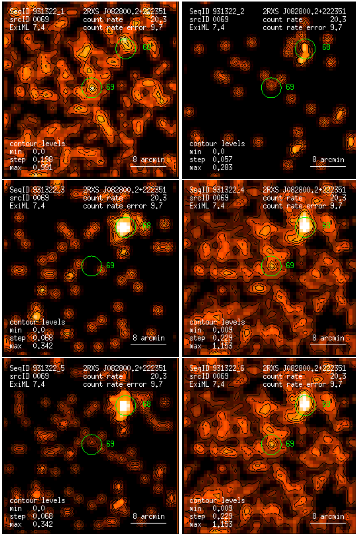
Figure 69: RASS 931322: detection 0069: band rate images, Gaussian filter: (1) PSPC channels 11 – 41, (2) 52 – 90, (3) 91 – 201, (4) 11 – 235, (5) 52 – 201, (6) 11 – 201. Broad band rates in counts/ks. Band rate contour levels in counts/ks/arcmin 2 .
