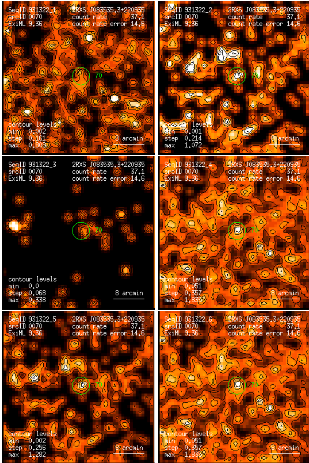
Figure 70: RASS 931322: detection 0070: band rate images, Gaussian filter: (1) PSPC channels 11 – 41, (2) 52 – 90, (3) 91 – 201, (4) 11 – 235, (5) 52 – 201, (6) 11 – 201. Broad band rates in counts/ks. Band rate contour levels in counts/ks/arcmin 2 .
