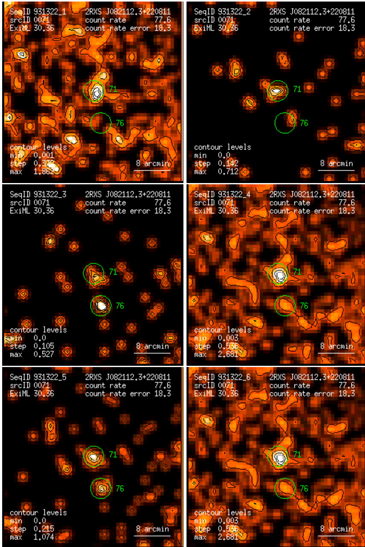
Figure 71: RASS 931322: detection 0071: band rate images, Gaussian filter: (1) PSPC channels 11 – 41, (2) 52 – 90, (3) 91 – 201, (4) 11 – 235, (5) 52 – 201, (6) 11 – 201. Broad band rates in counts/ks. Band rate contour levels in counts/ks/arcmin 2 .
