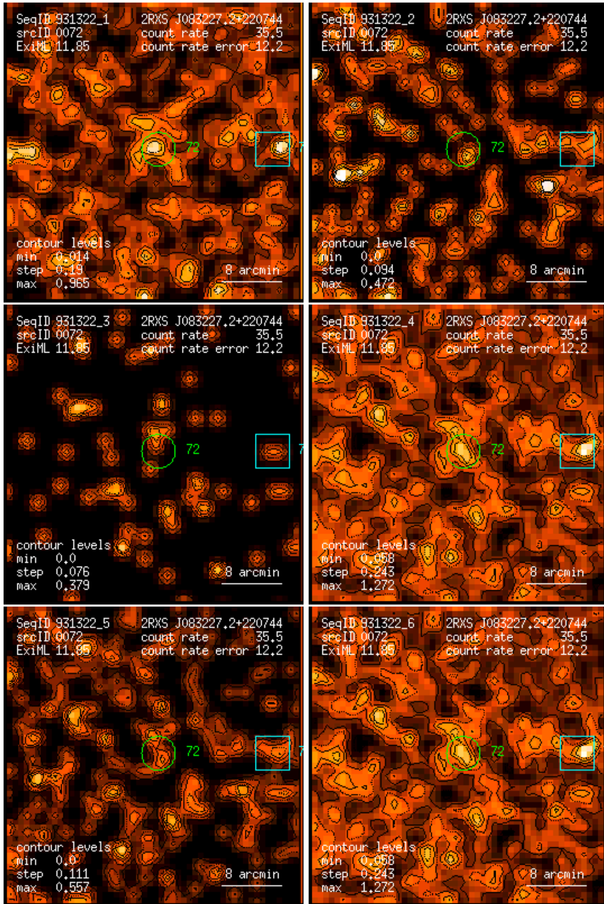
Figure 72: RASS 931322: detection 0072: band rate images, Gaussian filter: (1) PSPC channels 11 – 41, (2) 52 – 90, (3) 91 – 201, (4) 11 – 235, (5) 52 – 201, (6) 11 – 201. Broad band rates in counts/ks. Band rate contour levels in counts/ks/arcmin 2 .
