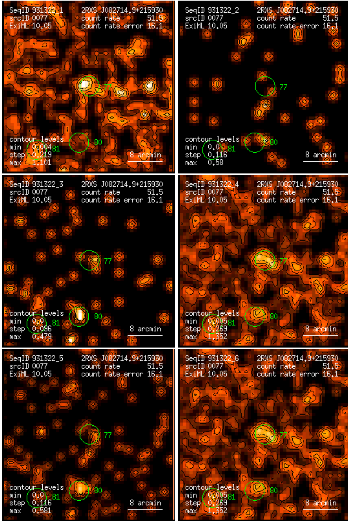
Figure 77: RASS 931322: detection 0077: band rate images, Gaussian filter: (1) PSPC channels 11 – 41, (2) 52 – 90, (3) 91 – 201, (4) 11 – 235, (5) 52 – 201, (6) 11 – 201. Broad band rates in counts/ks. Band rate contour levels in counts/ks/arcmin 2 .
