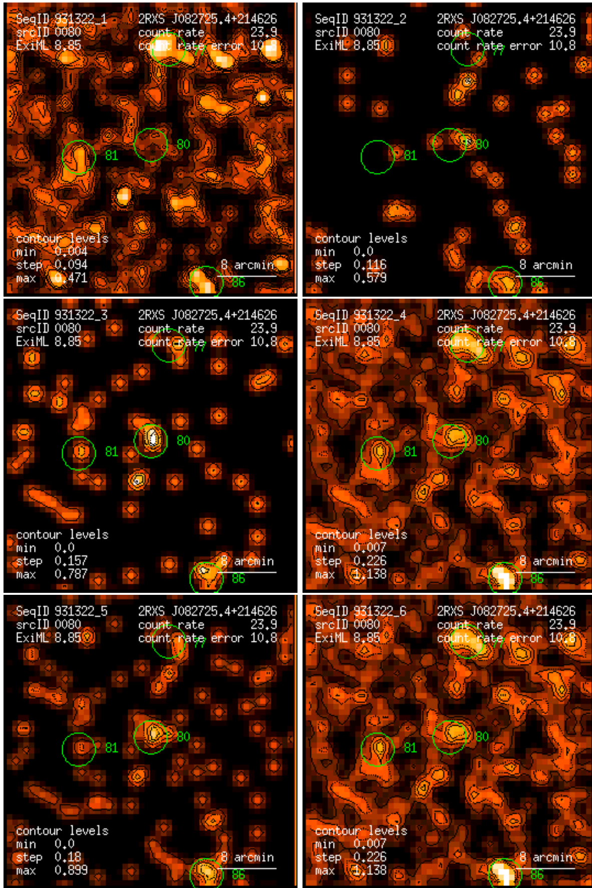
Figure 80: RASS 931322: detection 0080: band rate images, Gaussian filter: (1) PSPC channels 11 – 41, (2) 52 – 90, (3) 91 – 201, (4) 11 – 235, (5) 52 – 201, (6) 11 – 201. Broad band rates in counts/ks. Band rate contour levels in counts/ks/arcmin 2 .
