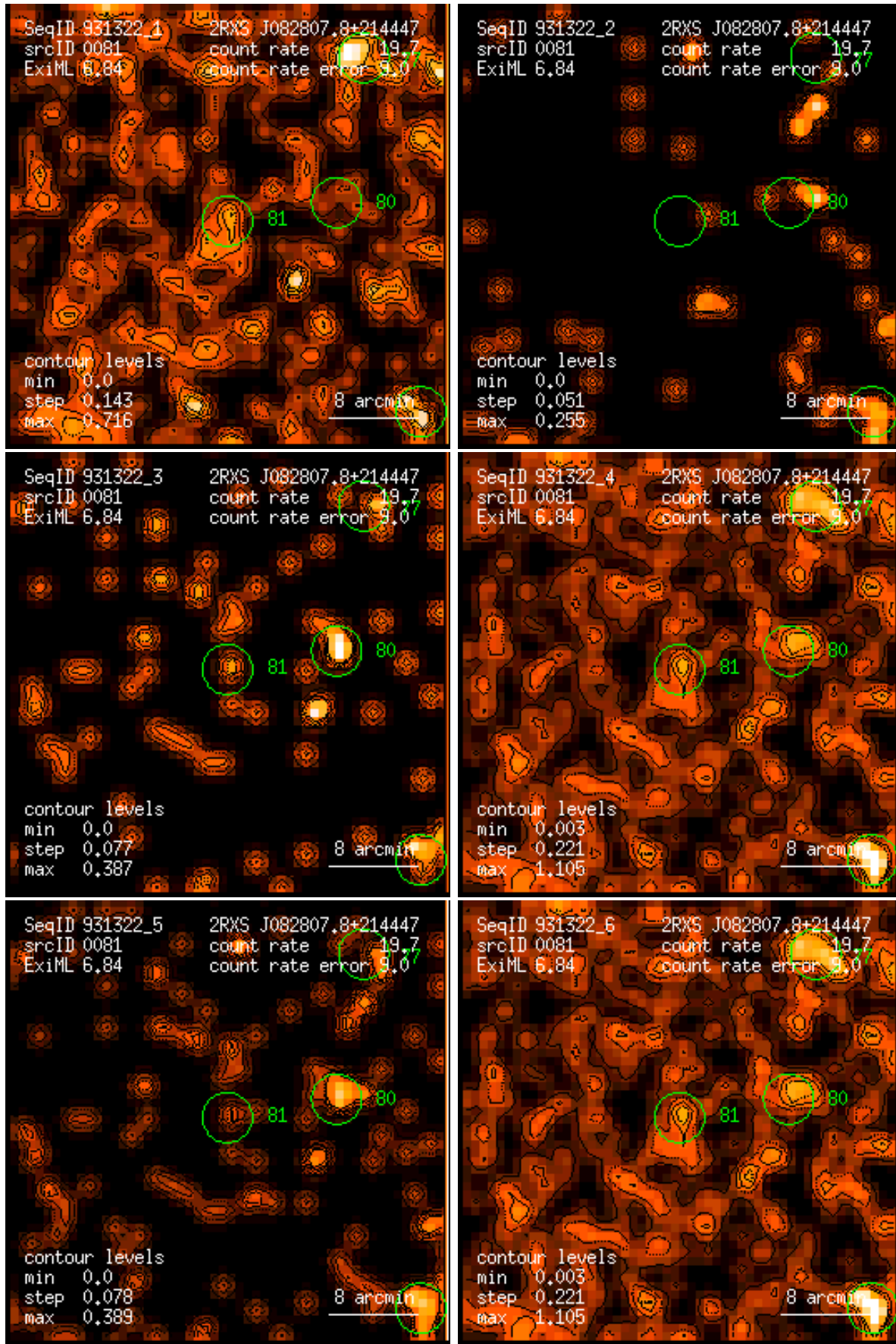
Figure 81: RASS 931322: detection 0081: band rate images, Gaussian filter: (1) PSPC channels 11 – 41, (2) 52 – 90, (3) 91 – 201, (4) 11 – 235, (5) 52 – 201, (6) 11 – 201. Broad band rates in counts/ks. Band rate contour levels in counts/ks/arcmin 2 .
