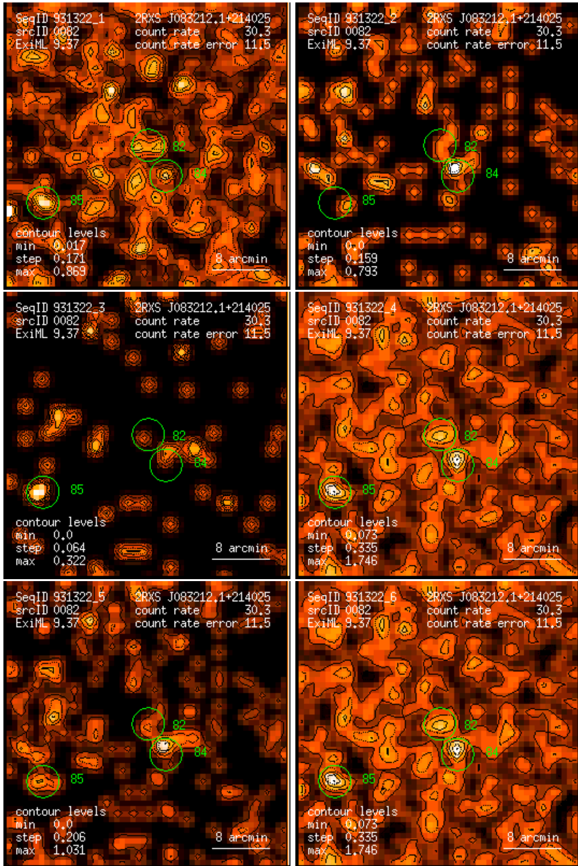
Figure 82: RASS 931322: detection 0082: band rate images, Gaussian filter: (1) PSPC channels 11 – 41, (2) 52 – 90, (3) 91 – 201, (4) 11 – 235, (5) 52 – 201, (6) 11 – 201. Broad band rates in counts/ks. Band rate contour levels in counts/ks/arcmin 2 .
