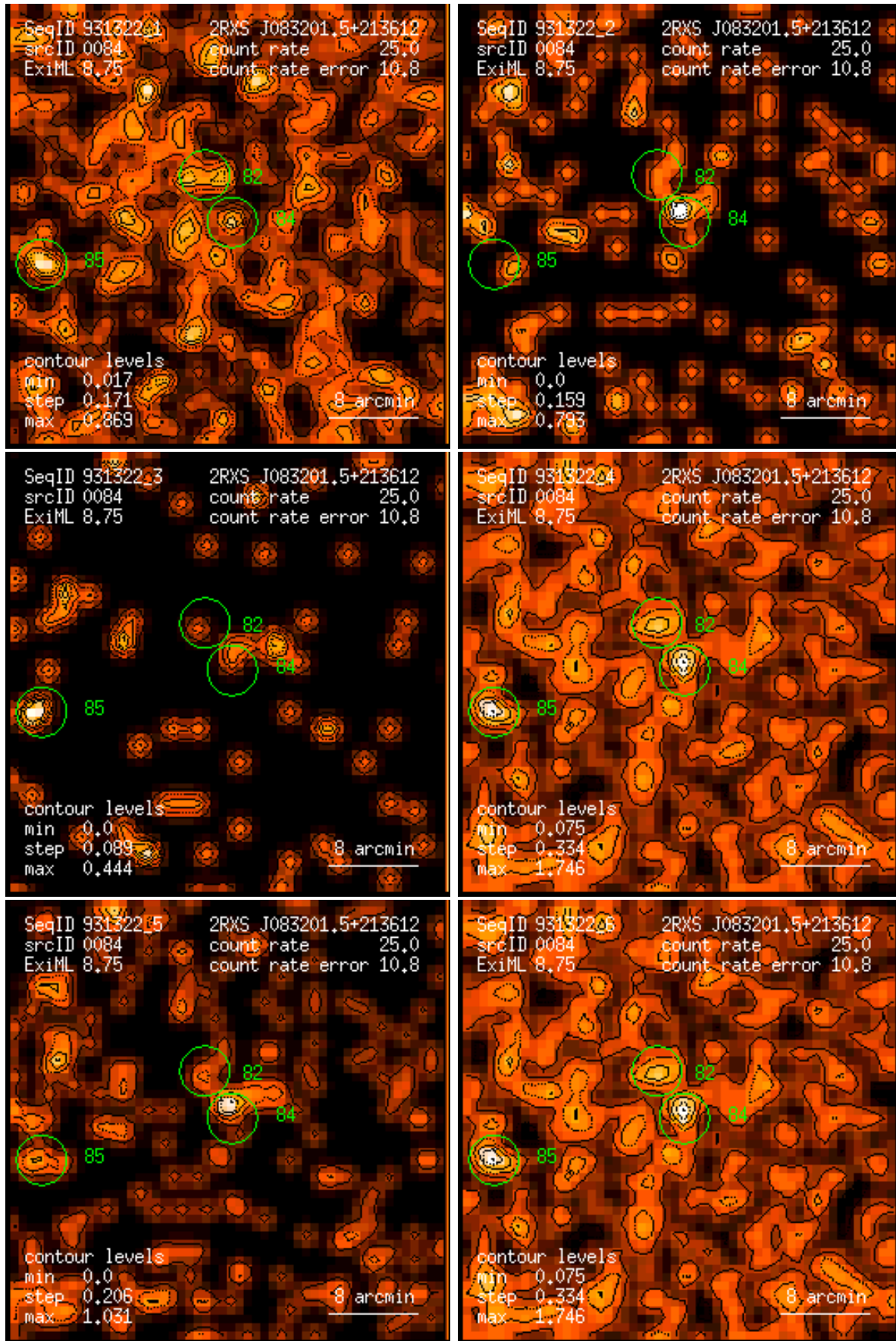
Figure 84: RASS 931322: detection 0084: band rate images, Gaussian filter: (1) PSPC channels 11 – 41, (2) 52 – 90, (3) 91 – 201, (4) 11 – 235, (5) 52 – 201, (6) 11 – 201. Broad band rates in counts/ks. Band rate contour levels in counts/ks/arcmin 2 .
