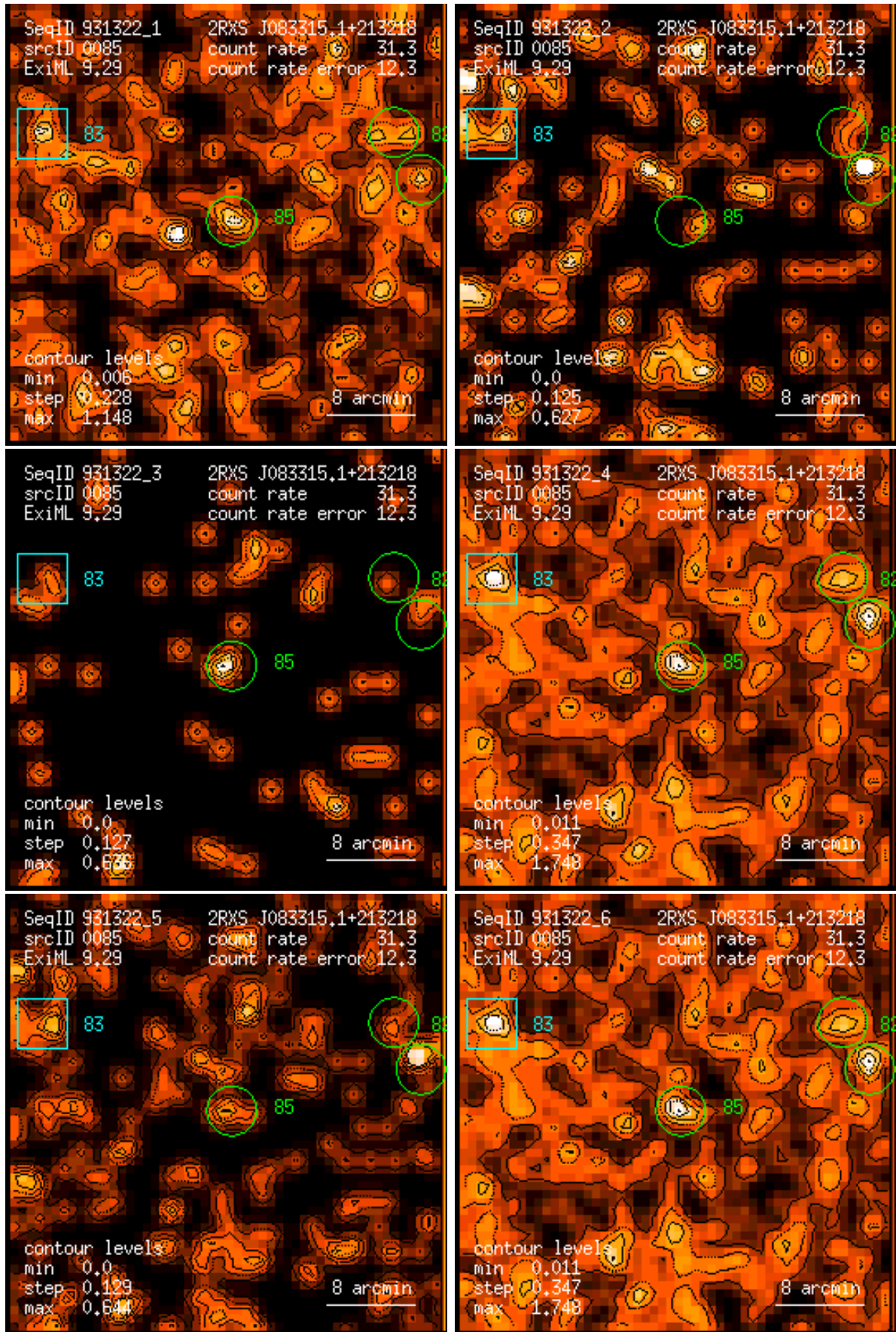
Figure 85: RASS 931322: detection 0085: band rate images, Gaussian filter: (1) PSPC channels 11 – 41, (2) 52 – 90, (3) 91 – 201, (4) 11 – 235, (5) 52 – 201, (6) 11 – 201. Broad band rates in counts/ks. Band rate contour levels in counts/ks/arcmin 2 .
