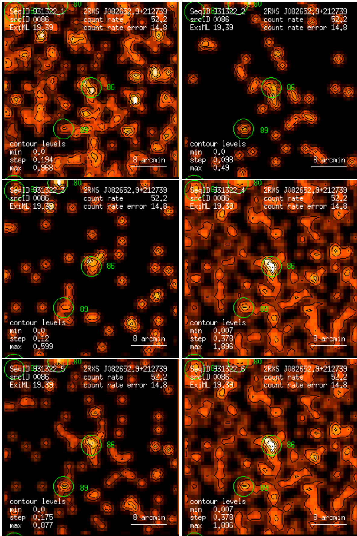
Figure 86: RASS 931322: detection 0086: band rate images, Gaussian filter: (1) PSPC channels 11 – 41, (2) 52 – 90, (3) 91 – 201, (4) 11 – 235, (5) 52 – 201, (6) 11 – 201. Broad band rates in counts/ks. Band rate contour levels in counts/ks/arcmin 2 .
